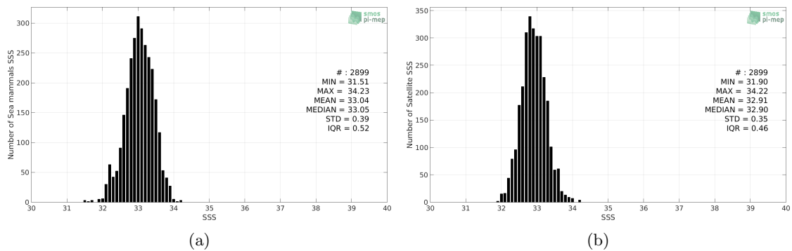
Figure 2: Histograms of SSS from Sea mammals (a) and SMAP-L3-RSS-V4-MONTHLY (b) considering all match-up pairs per bins of 0.1 over the Pacific Ocean Pi-MEP region and for the full satellite product period.
