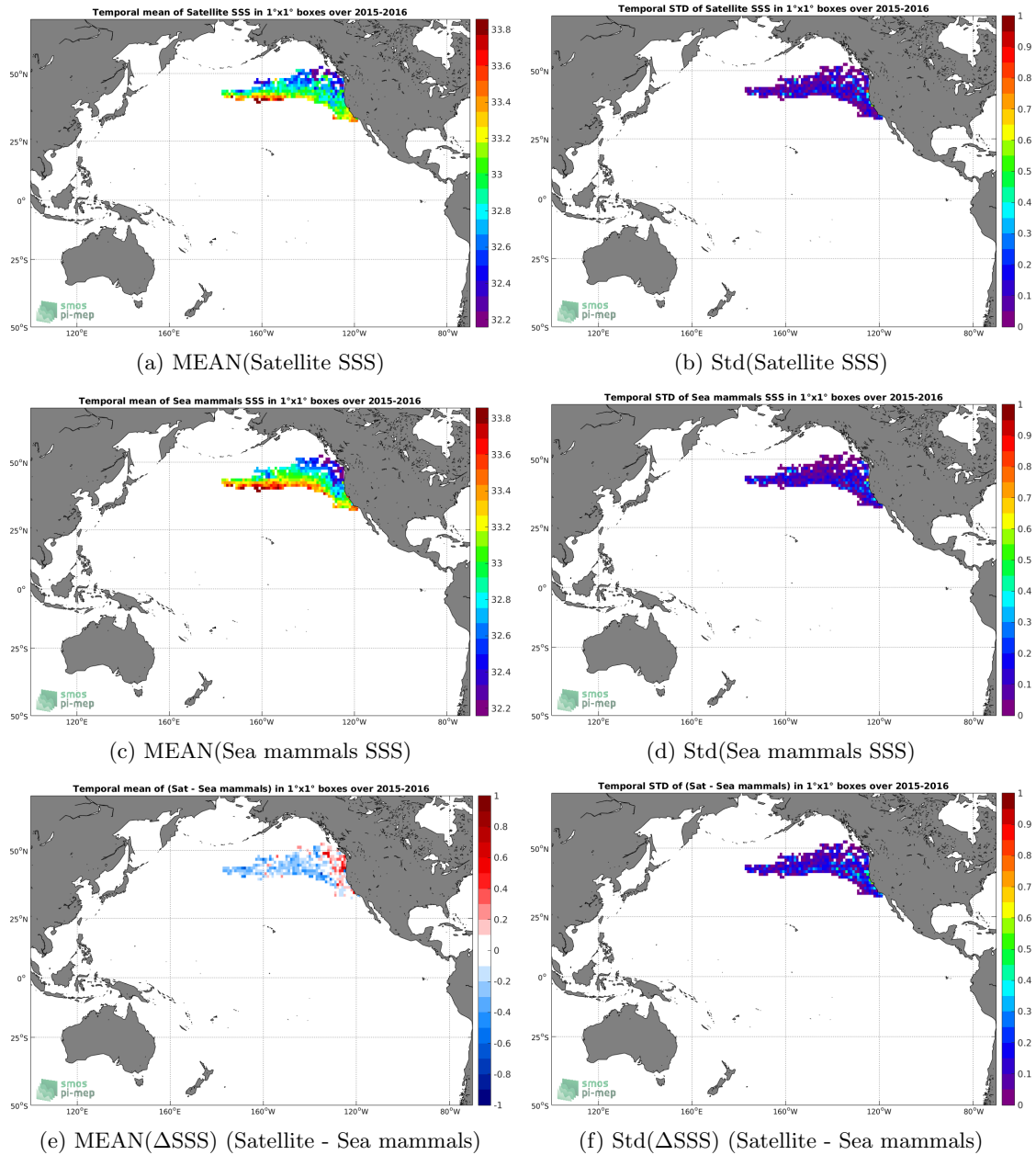
Figure 6: Temporal mean (left) and Std (right) of SSS from SMAP-L3-RSS-V4-MONTHLY (top), Sea mammals (middle), and of \Delta SSS (Satellite - Sea mammals). Only match-up pairs are used to generate these maps.
