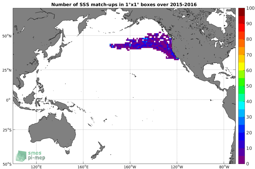
Figure 4: Number of SSS match-ups between Sea mammals SSS and the SMAP-L3-RSS-V4-MONTHLY SSS product for the Pacific Ocean Pi-MEP region over 1°x1° boxes and for the full satellite product period.
