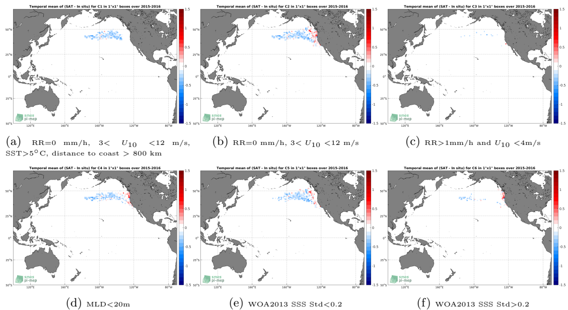
Figure 12: Temporal mean gridded over spatial boxes of size 1^\circ \times 1^\circ of \Delta SSS (SMAP-L3-RSS-V4-MONTHLY - Sea mammals) for 6 different subdatasets corresponding to:RR=0 mm/h, 3 < U_{10} < 12 m/s, SST >5^\circ C, distance to coast > 800 km (a), RR=0 mm/h, 3 < U_{10} < 12 m/s (b), RR >1 mm/h and U_{10} < 4 m/s (c),MLD <20 m (d),WOA2013 SSS Std <0.2 (e),WOA2013 SSS Std >0.2 (f).
