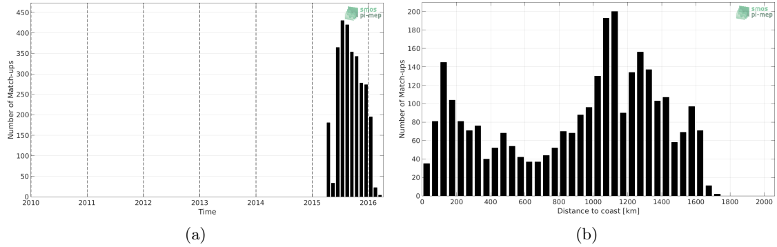
Figure 1: Number of match-ups between Sea mammals and SMAP-L3-RSS-V4-MONTHLY SSS as a function of time (a) and as function of the distance to coast (b) over the Pacific Ocean Pi-MEP region and for the full satellite product period.
