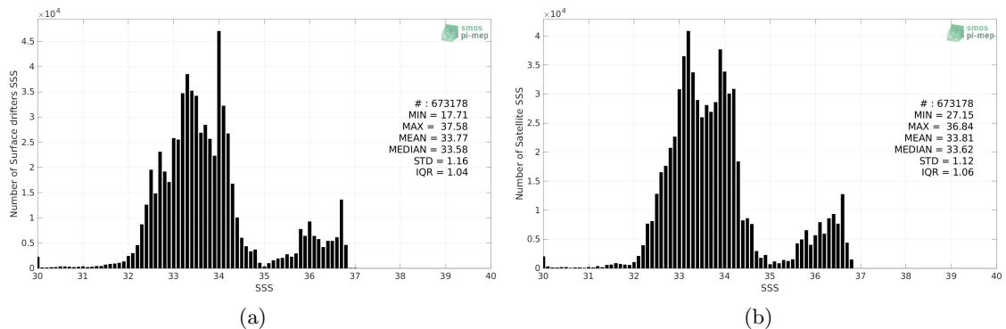
Figure 2: Histograms of SSS from Surface drifters (a) and SMAP SSS L3 v4 - Monthly (RSS) (b) considering all match-up pairs per bins of 0.1 over the Pacific Ocean Pi-MEP region and for the full satellite product period.
