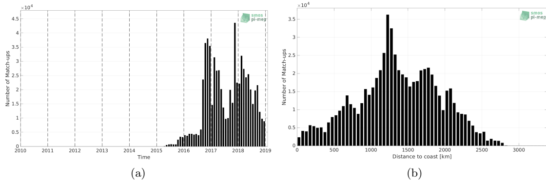
Figure 1: Number of match-ups between Surface drifters and SMAP SSS L3 v4 - Monthly (RSS) SSS as a function of time (a) and as function of the distance to coast (b) over the Pacific Ocean Pi-MEP region and for the full satellite product period.
