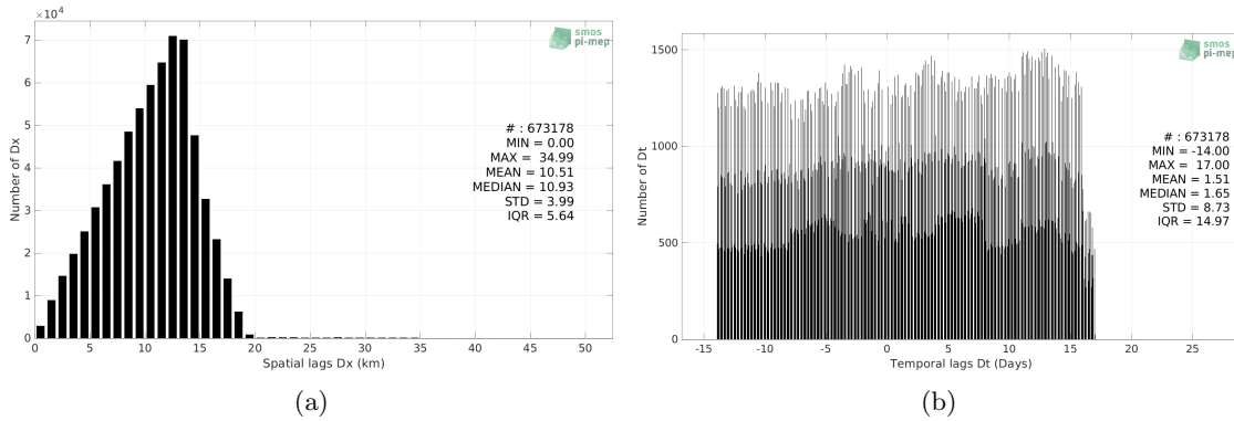
Figure 4: Histograms of the spatial (a) and temporal (b) lags between the location/time of the Surface drifters measurement and the date of the corresponding SMAP SSS L3 v4 - Monthly (RSS) SSS pixel.
