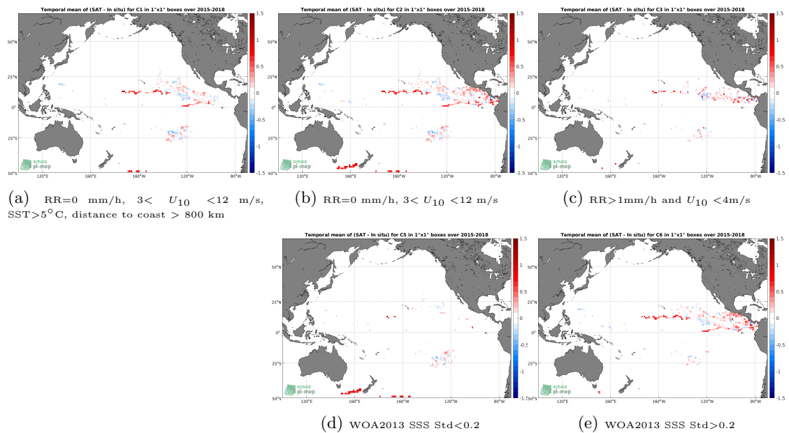
Figure 11: Temporal mean gridded over spatial boxes of size 1^\circ \times 1^\circ of \Delta SSS (SMAP SSS L3 v4 - Monthly (RSS) - Surface drifters) for 5 different subdatasets corresponding to: RR=0 mm/h, 3 < U_{10} < 12 m/s, SST > 5°C, distance to coast > 800 km (a), RR=0 mm/h, 3 < U_{10} < 12 m/s (b), RR > 1mm/h and U_{10} < 4 m/s (c), WOA2013 SSS Std < 0.2 (d), WOA2013 SSS Std > 0.2 (e).
