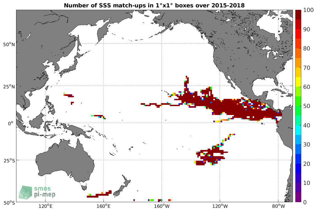
Figure 3: Number of SSS match-ups between Surface drifters SSS and the SMAP SSS L3 v4 - Monthly (RSS) SSS product for the Pacific Ocean Pi-MEP region over 1°x1° boxes and for the full satellite product period.
