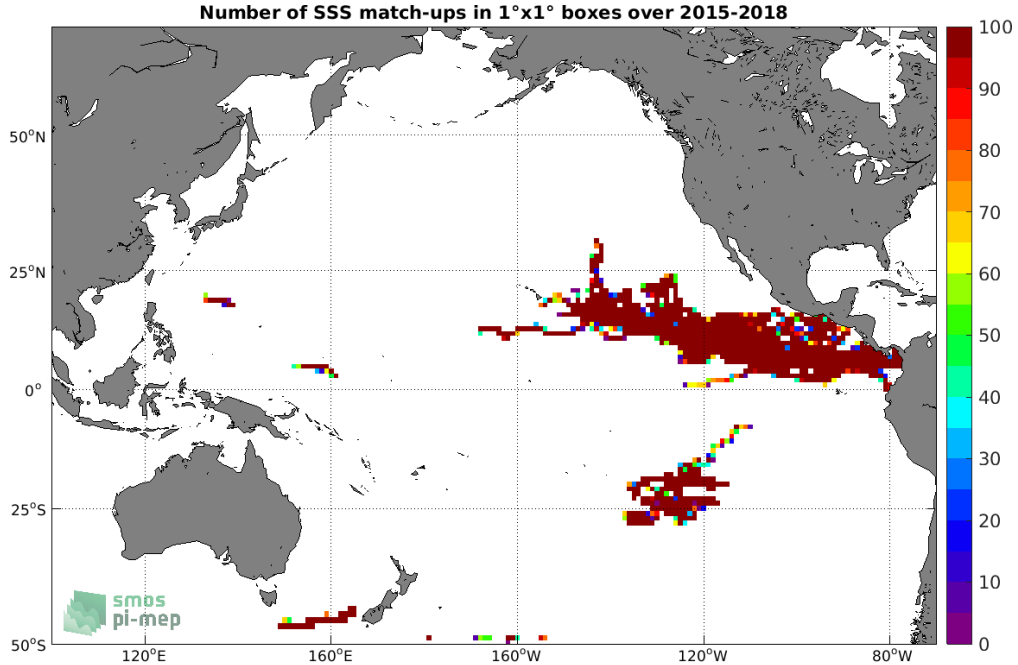
Figure 3: Number of SSS match-ups between Surface drifters SSS and the SMAP SSS L3 v4 - Monthly (RSS) SSS product for the Pacific Ocean Pi-MEP region over 1°x1° boxes and for the full satellite product period.
