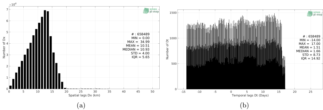
Figure 4: Histograms of the spatial (a) and temporal (b) lags between the time of the Surface drifters measurements and the date of the corresponding SMAP SSS L3 v4 - Monthly (RSS) SSS product.
