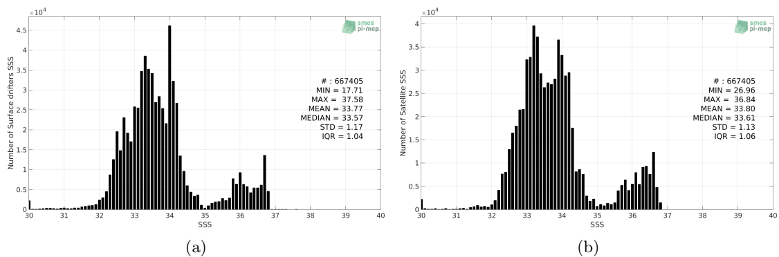
Figure 2: Histograms of SSS from Surface drifters (a) and SMAP-L3-RSS-V4-MONTHLY (b) considering all match-up pairs per bins of 0.1 over the Pacific Ocean Pi-MEP region and for the full satellite product period.
