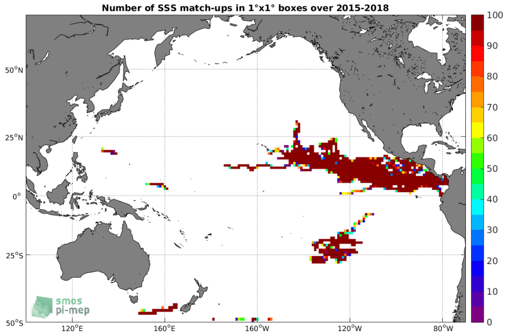
Figure 3: Number of SSS match-ups between Surface drifters SSS and the SMAP-L3-RSS-V4-MONTHLY SSS product for the Pacific Ocean Pi-MEP region over 1^{\circ} \times 1^{\circ} boxes and for the full satellite product period.
