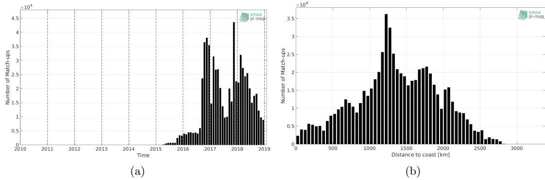
Figure 1: Number of match-ups between Surface drifters and SMAP-L3-RSS-V4-MONTHLY SSS as a function of time (a) and as function of the distance to coast (b) over the Pacific Ocean Pi-MEP region and for the full satellite product period.
