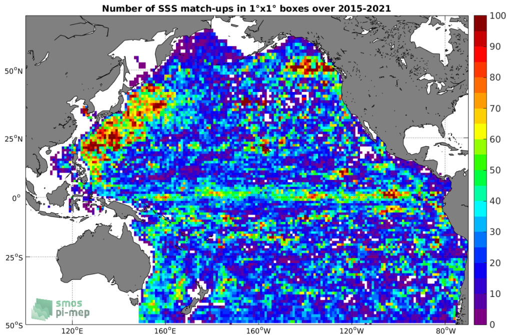
Figure 4: Number of SSS match-ups between Argo SSS and the SMAP SSS L3 v4 - Monthly (RSS) SSS product for the Pacific Ocean Pi-MEP region over 1^\circ \times 1^\circ boxes and for the full satellite product period.
