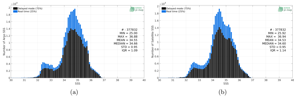
Figure 2: Histograms of SSS from Argo (a) and SMAP SSS L3 v4 - Monthly (RSS) (b) considering all match-up pairs per bins of 0.1 over the Pacific Ocean Pi-MEP region and for the full satellite product period.
