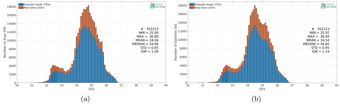
Figure 2: Histograms of SSS from Argo (a) and SMAP SSS L3 v4 - Monthly (RSS) (b) considering all match-up pairs per bins of 0.1 over the Pacific Ocean Pi-MEP region and for the full satellite product period.
