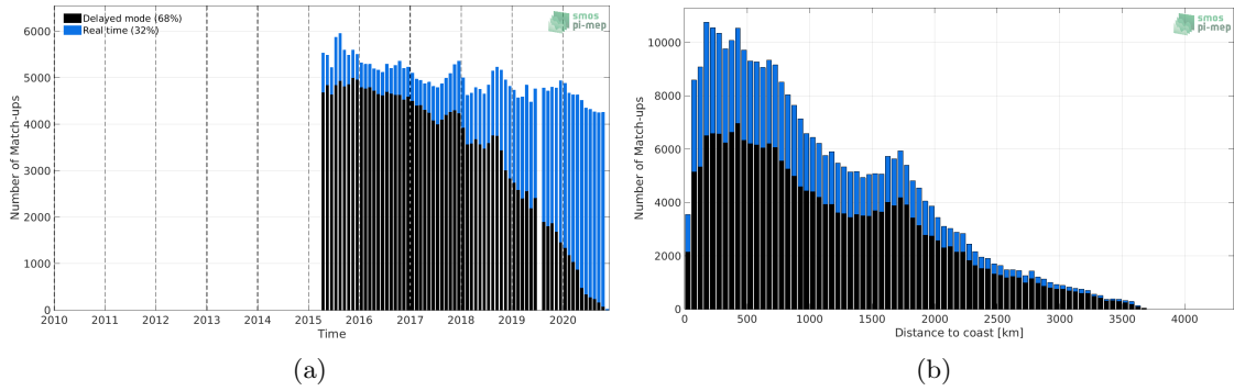
Figure 1: Number of match-ups between Argo and SMAP SSS L3 v4 - Monthly (RSS) SSS as a function of time (a) and as function of the distance to coast (b) over the Pacific Ocean Pi-MEP region and for the full satellite product period.
