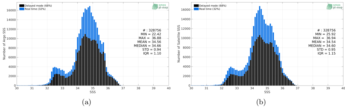
Figure 2: Histograms of SSS from Argo (a) and SMAP SSS L3 v4 - Monthly (RSS) (b) considering all match-up pairs per bins of 0.1 over the Pacific Ocean Pi-MEP region and for the full satellite product period.
