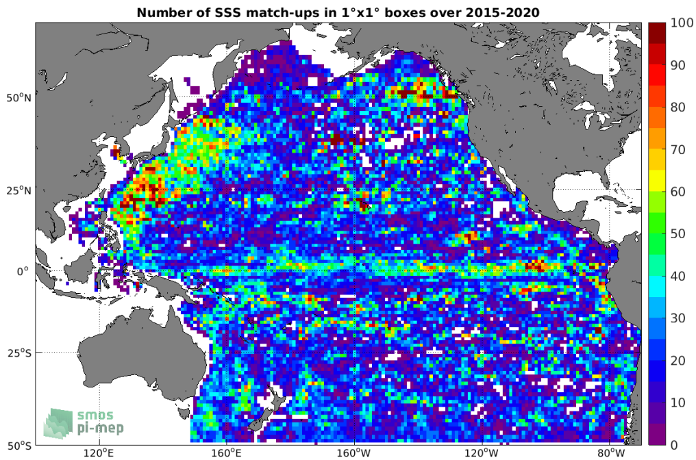
Figure 4: Number of SSS match-ups between Argon SSS and the SMAP SSS L3 v4 - Monthly (RSS) SSS product for the Pacific Ocean Pi-MEP region over 1^\circ \times 1^\circ boxes and for the full satellite product period.
