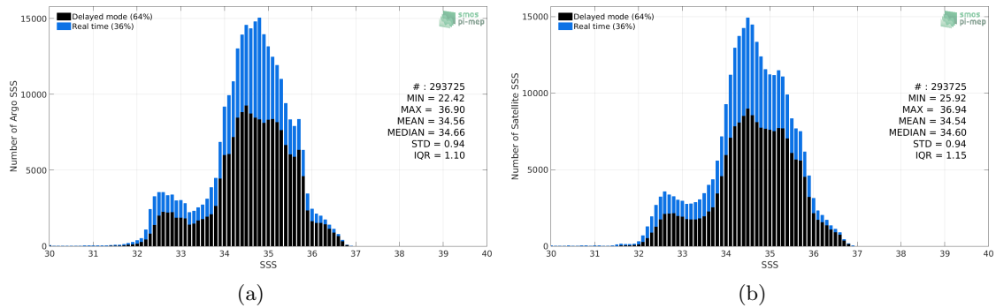
Figure 2: Histograms of SSS from Argo (a) and SMAP-L3-RSS-V4-MONTHLY (b) considering all match-up pairs per bins of 0.1 over the Pacific Ocean Pi-MEP region and for the full satellite product period.
