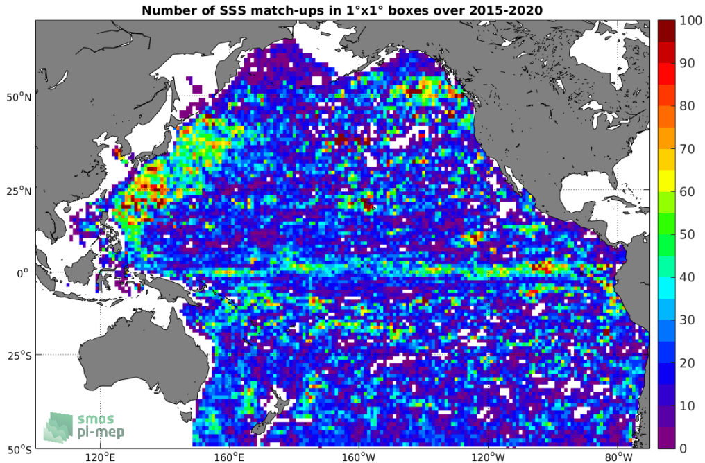
Figure 4: Number of SSS match-ups between Argo SSS and the SMAP-L3-RSS-V4-MONTHLY SSS product for the Pacific Ocean Pi-MEP region over 1°x1° boxes and for the full satellite product period.
