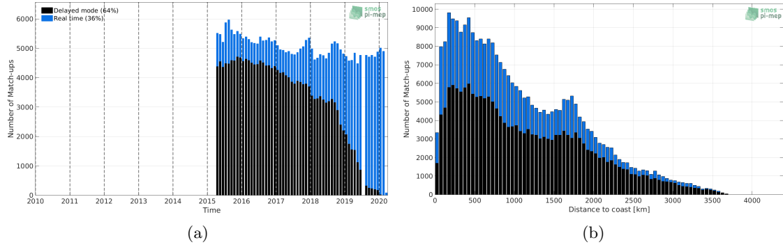
Figure 1: Number of match-ups between Argo and SMAP-L3-RSS-V4-MONTHLY SSS as a function of time (a) and as function of the distance to coast (b) over the Pacific Ocean Pi-MEP region and for the full satellite product period.
