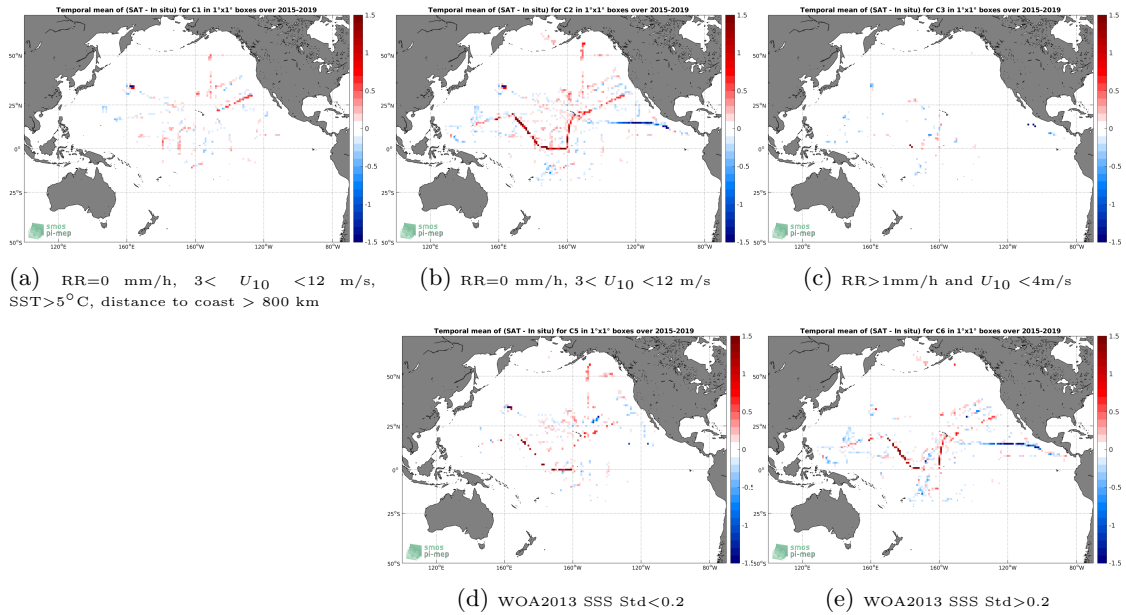
Figure 12: Temporal mean gridded over spatial boxes of size 1^\circ \times 1^\circ of \Delta SSS (SMAP-L3-RSS-V3-8DAY-RUNNING-70KM - TSG-SAMOS) for 5 different subdatasets corresponding to: RR=0 mm/h, 3 < U_{10} < 12 m/s, SST > 5^\circ C , distance to coast > 800 km (a), RR=0 mm/h, 3 < U_{10} < 12 m/s (b), RR > 1 mm/h and U_{10} < 4 m/s (c), WOA2013 SSS Std < 0.2 (d), WOA2013 SSS Std > 0.2 (e).
