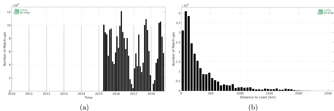
Figure 1: Number of match-ups between TSG-SAMOS and SMAP-L3-RSS-V3-8DAY-RUNNING-70KM SSS as a function of time (a) and as function of the distance to coast (b) over the Pacific Ocean Pi-MEP region and for the full satellite product period.
