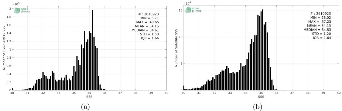
Figure 2: Histograms of SSS from TSG-SAMOS (a) and SMAP-L3-RSS-V3-8DAY-RUNNING-70KM (b) considering all match-up pairs per bins of 0.1 over the Pacific Ocean Pi-MEP region and for the full satellite product period.
