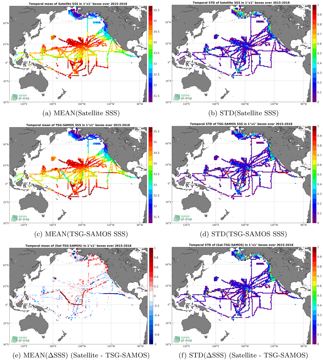
Figure 6: Temporal mean (left) and STD (right) of SSS from SMAP-L3-RSS-V3-8DAY-RUNNING-70KM (top), TSG-SAMOS (middle), and of \Delta SSS (Satellite - TSG-SAMOS). Only match-up pairs are used to generate these maps.
