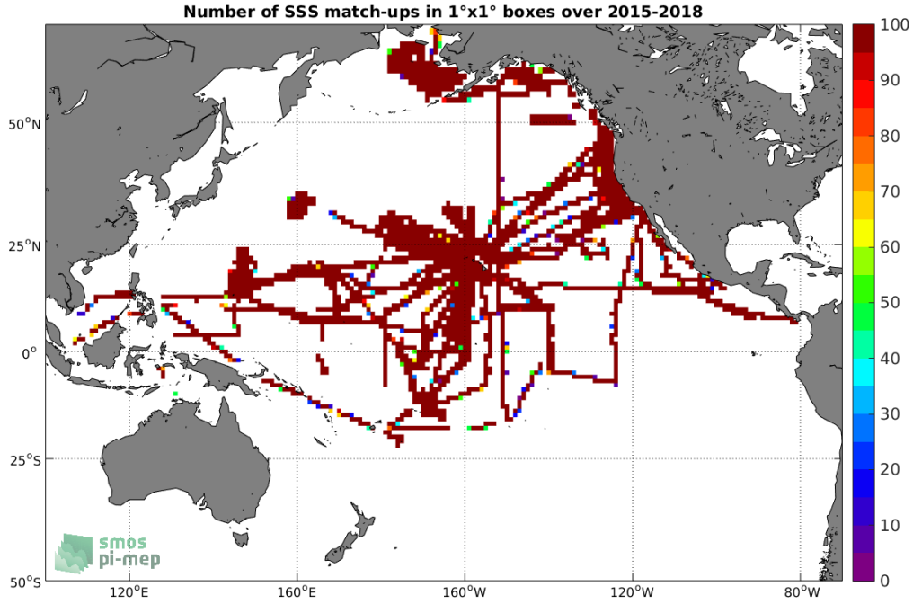
Figure 4: Number of SSS match-ups between TSG-SAMOS SSS and the SMAP-L3-RSS-V3-8DAY-RUNNING-70KM SSS product for the Pacific Ocean Pi-MEP region over 1^\circ \times 1^\circ boxes and for the full satellite product period.
