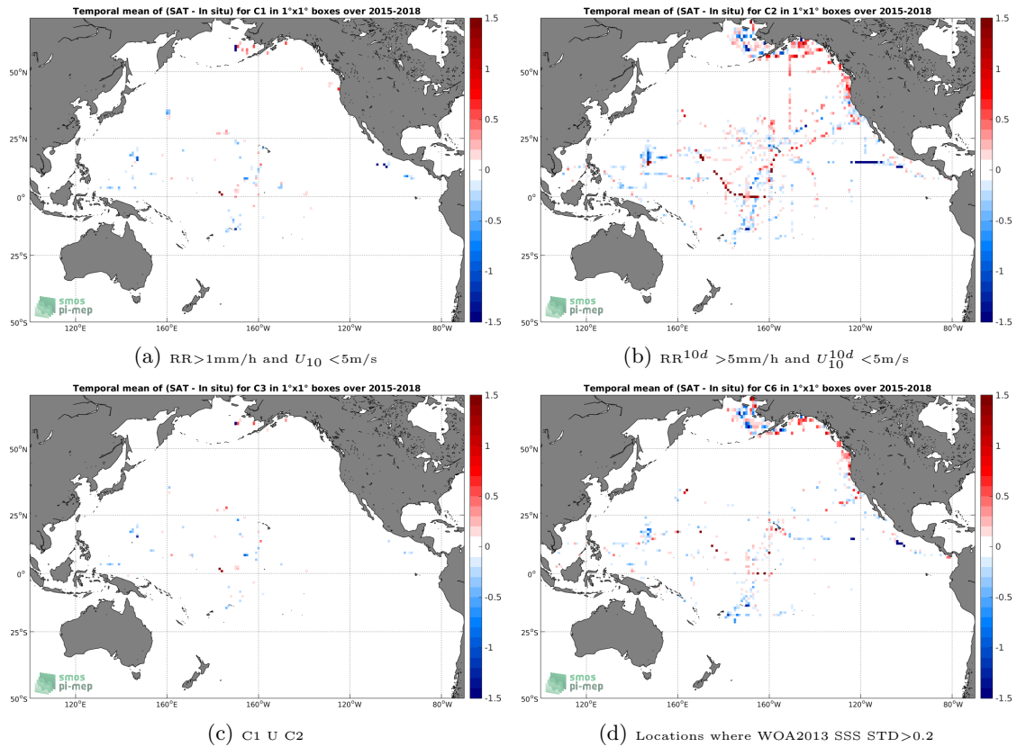
Figure 12: Temporal mean gridded over spatial boxes of size 1^\circ \times 1^\circ of \Delta SSS (SMAP-L3-RSS-V3-8DAY-RUNNING-70KM - TSG-SAMOS) for 4 different subdatasets corresponding to: RR > 1mm/h and U_{10} < 5\text{m/s} (a), RR^{10d} > 5\text{mm/h} and U_{10}^{10d} < 5\text{m/s} (b), C1 U C2 (c), Locations where WOA2013 SSS STD > 0.2 (d).
