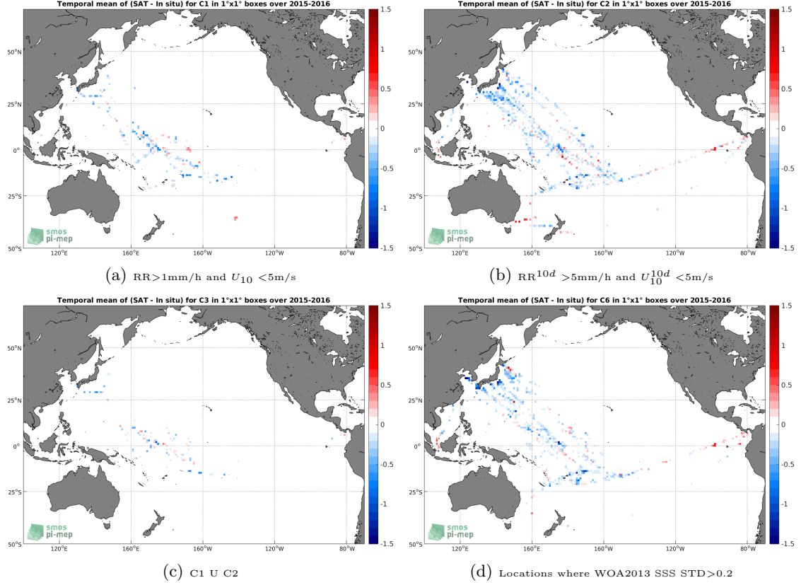
Figure 12: Temporal mean gridded over spatial boxes of size 1^\circ \times 1^\circ of \Delta SSS (SMAP-L3-RSS-V3-8DAY-RUNNING-70KM - TSG-LEGOS-DM) for 4 different subdatasets corresponding to: RR > 1mm/h and U_{10} < 5\text{m/s} (a), RR^{10d} > 5\text{mm/h} and U_{10}^{10d} < 5\text{m/s} (b), C1 U C2 (c), Locations where WOA2013 SSS STD > 0.2 (d).
