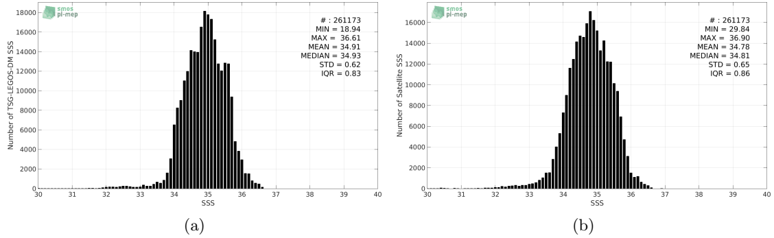
Figure 2: Histograms of SSS from TSG-LEGOS-DM (a) and SMAP-L3-RSS-V3-8DAY-RUNNING-70KM (b) considering all match-up pairs per bins of 0.1 over the Pacific Ocean Pi-MEP region and for the full satellite product period.
