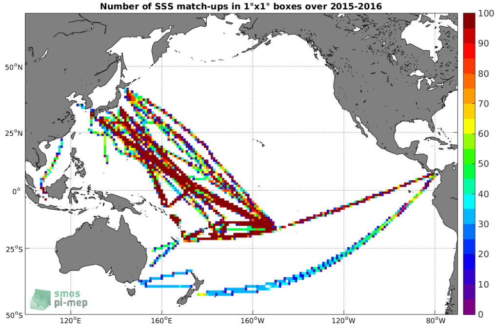
Figure 4: Number of SSS match-ups between TSG-LEGOS-DM SSS and the SMAP-L3-RSS-V3-8DAY-RUNNING-70KM SSS product for the Pacific Ocean Pi-MEP region over 1^\circ \times 1^\circ boxes and for the full satellite product period.
