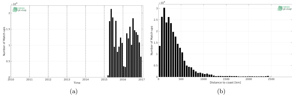
Figure 1: Number of match-ups between TSG-LEGOS-DM and SMAP-L3-RSS-V3-8DAY-RUNNING-70KM SSS as a function of time (a) and as function of the distance to coast (b) over the Pacific Ocean Pi-MEP region and for the full satellite product period.
