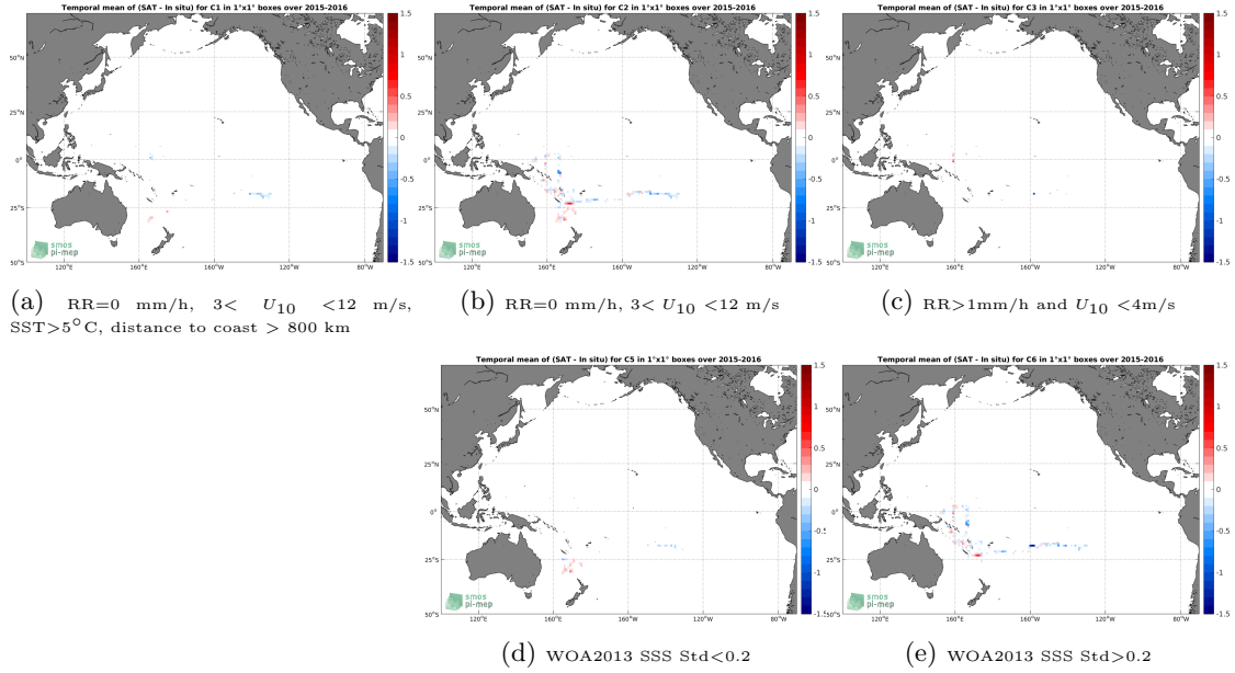
Figure 12: Temporal mean gridded over spatial boxes of size 1^\circ \times 1^\circ of \Delta SSS (SMAP-L3-RSS-V3-8DAY-RUNNING-70KM - TSG-GOSUD-Research-vessel) for 5 different subdatasets corresponding to:RR=0 mm/h, 3 < U_{10} < 12 m/s, SST >5^\circ C, distance to coast > 800 km (a), RR=0 mm/h, 3 < U_{10} < 12 m/s (b), RR >1 mm/h and U_{10} < 4 m/s (c), WOA2013 SSS Std <0.2 (d), WOA2013 SSS Std >0.2 (e).
