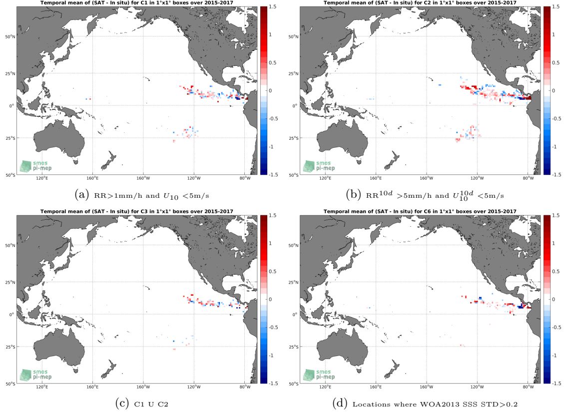
Figure 11: Temporal mean gridded over spatial boxes of size 1^\circ \times 1^\circ of \Delta SSS (SMAP-L3-RSS-V3-8DAY-RUNNING-70KM - Surface drifters) for 4 different subdatasets corresponding to: RR > 1\text{mm/h} and U_{10} < 5\text{m/s} (a), RR^{10d} > 5\text{mm/h} and U_{10}^{10d} < 5\text{m/s} (b), C1 U C2 (c), Locations where WOA2013 SSS STD > 0.2 (d).
