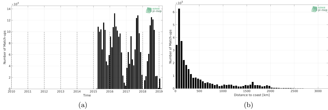
Figure 1: Number of match-ups between TSG-SAMOS and SMAP-L3-RSS-V3-8DAY-RUNNING-40KM SSS as a function of time (a) and as function of the distance to coast (b) over the Pacific Ocean Pi-MEP region and for the full satellite product period.
