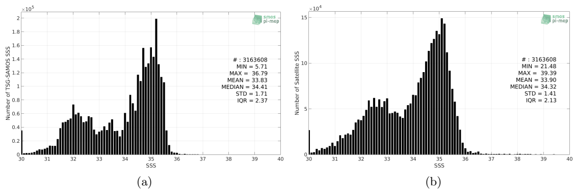
Figure 2: Histograms of SSS from TSG-SAMOS (a) and SMAP-L3-RSS-V3-8DAY-RUNNING-40KM (b) considering all match-up pairs per bins of 0.1 over the Pacific Ocean Pi-MEP region and for the full satellite product period.
