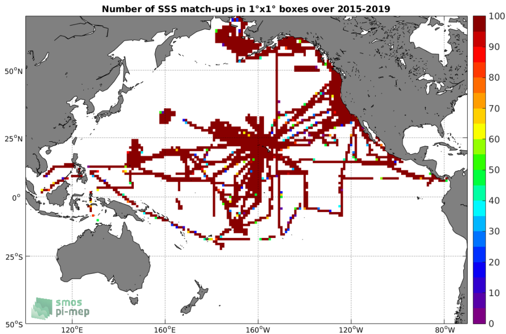
Figure 4: Number of SSS match-ups between TSG-SAMOS SSS and the SMAP-L3-RSS-V3-8DAY-RUNNING-40KM SSS product for the Pacific Ocean Pi-MEP region over 1^\circ \times 1^\circ boxes and for the full satellite product period.
