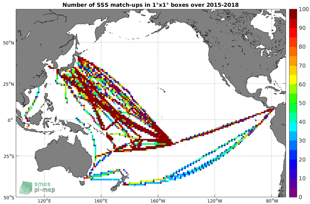
Figure 4: Number of SSS match-ups between TSG-LEGOS-DM SSS and the SMAP-L3-RSS-V3-8DAY-RUNNING-40KM SSS product for the Pacific Ocean Pi-MEP region over 1^\circ \times 1^\circ boxes and for the full satellite product period.
