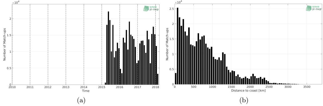
Figure 1: Number of match-ups between TSG-LEGOS-DM and SMAP-L3-RSS-V3-8DAY-RUNNING-40KM SSS as a function of time (a) and as function of the distance to coast (b) over the Pacific Ocean Pi-MEP region and for the full satellite product period.
