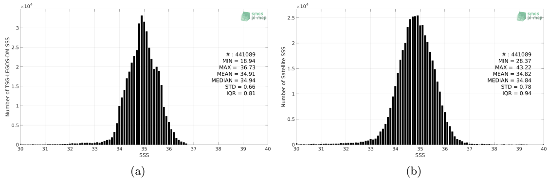
Figure 2: Histograms of SSS from TSG-LEGOS-DM (a) and SMAP-L3-RSS-V3-8DAY-RUNNING-40KM (b) considering all match-up pairs per bins of 0.1 over the Pacific Ocean Pi-MEP region and for the full satellite product period.
