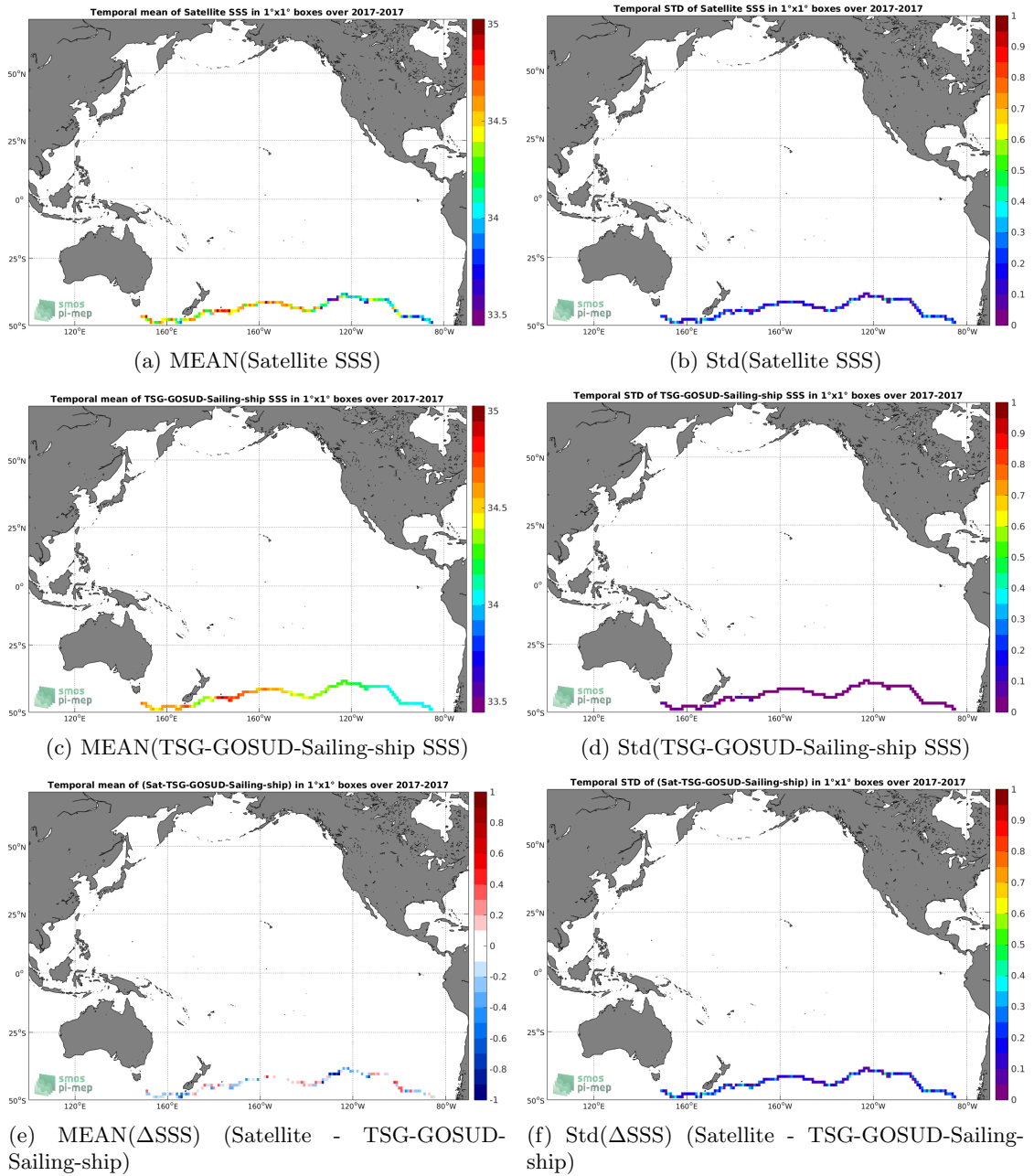
Figure 6: Temporal mean (left) and Std (right) of SSS from SMAP-L3-RSS-V3-8DAY-RUNNING-40KM (top), TSG-GOSUD-Sailing-ship (middle), and of \Delta SSS (Satellite - TSG-GOSUD-Sailing-ship). Only match-up pairs are used to generate these maps.
