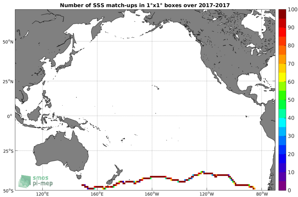
Figure 4: Number of SSS match-ups between TSG-GOSUD-Sailing-ship SSS and the SMAP-L3-RSS-V3-8DAY-RUNNING-40KM SSS product for the Pacific Ocean Pi-MEP region over 1^\circ \times 1^\circ boxes and for the full satellite product period.
