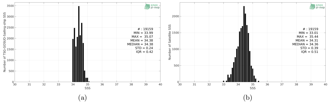
Figure 2: Histograms of SSS from TSG-GOSUD-Sailing-ship (a) and SMAP-L3-RSS-V3-8DAY-RUNNING-40KM (b) considering all match-up pairs per bins of 0.1 over the Pacific Ocean Pi-MEP region and for the full satellite product period.
