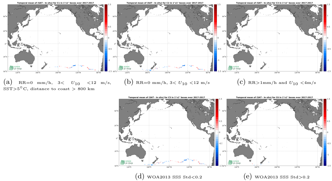
Figure 12: Temporal mean gridded over spatial boxes of size 1^\circ \times 1^\circ of \Delta SSS (SMAP-L3-RSS-V3-8DAY-RUNNING-40KM - TSG-GOSUD-Sailing-ship) for 5 different subdatasets corresponding to:RR=0 mm/h, 3 < U_{10} < 12 m/s, SST >5^\circ C, distance to coast > 800 km (a), RR=0 mm/h, 3 < U_{10} < 12 m/s (b), RR >1 mm/h and U_{10} < 4 m/s (c), WOA2013 SSS Std <0.2 (d), WOA2013 SSS Std >0.2 (e).
