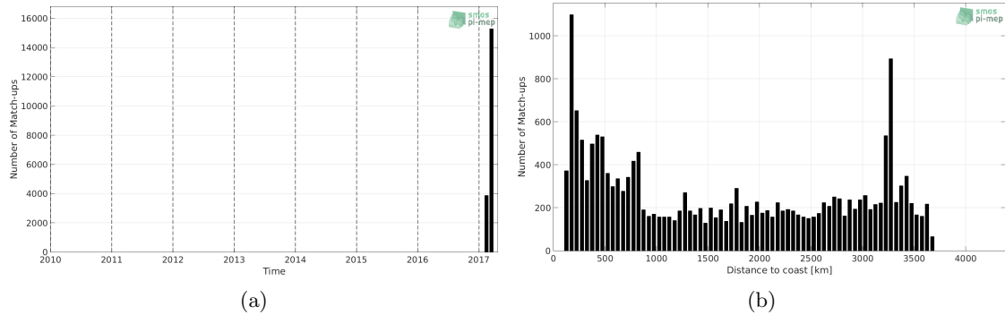
Figure 1: Number of match-ups between TSG-GOSUD-Sailing-ship and SMAP-L3-RSS-V3-8DAY-RUNNING-40KM SSS as a function of time (a) and as function of the distance to coast (b) over the Pacific Ocean Pi-MEP region and for the full satellite product period.
