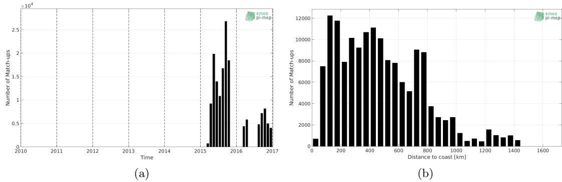
Figure 1: Number of match-ups between TSG-GOSUD-Research-vessel and SMAP-L3-RSS-V3-8DAY-RUNNING-40KM SSS as a function of time (a) and as function of the distance to coast (b) over the Pacific Ocean Pi-MEP region and for the full satellite product period.
