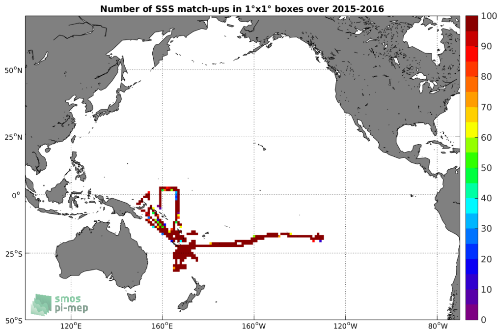
Figure 4: Number of SSS match-ups between TSG-GOSUD-Research-vessel SSS and the SMAP-L3-RSS-V3-8DAY-RUNNING-40KM SSS product for the Pacific Ocean Pi-MEP region over 1^\circ \times 1^\circ boxes and for the full satellite product period.
