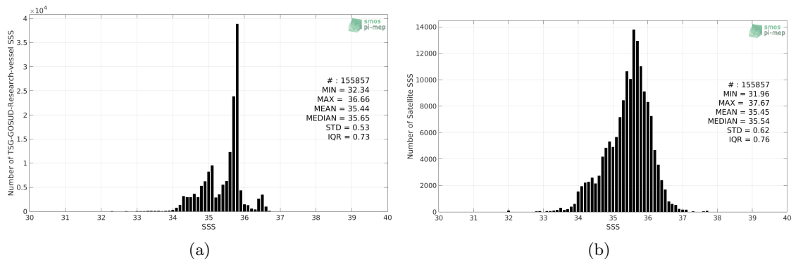
Figure 2: Histograms of SSS from TSG-GOSUD-Research-vessel (a) and SMAP-L3-RSS-V3-8DAY-RUNNING-40KM (b) considering all match-up pairs per bins of 0.1 over the Pacific Ocean Pi-MEP region and for the full satellite product period.
