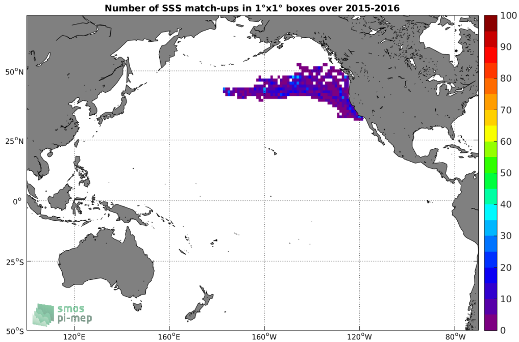
Figure 4: Number of SSS match-ups between Sea mammals SSS and the SMAP-L3-RSS-V3-8DAY-RUNNING-40KM SSS product for the Pacific Ocean Pi-MEP region over 1^\circ \times 1^\circ boxes and for the full satellite product period.
