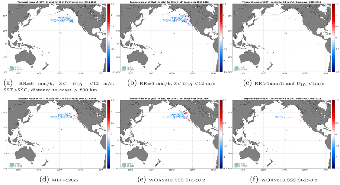
Figure 12: Temporal mean gridded over spatial boxes of size 1^\circ \times 1^\circ of \Delta SSS (SMAP-L3-RSS-V3-8DAY-RUNNING-40KM - Sea mammals) for 6 different subdatasets corresponding to: RR=0 mm/h, 3 < U_{10} < 12 m/s, SST > 5^\circ C , distance to coast > 800 km (a), RR=0 mm/h, 3 < U_{10} < 12 m/s (b), RR > 1 mm/h and U_{10} < 4 m/s (c), MLD < 20 m (d), WOA2013 SSS Std < 0.2 (e), WOA2013 SSS Std > 0.2 (f).
