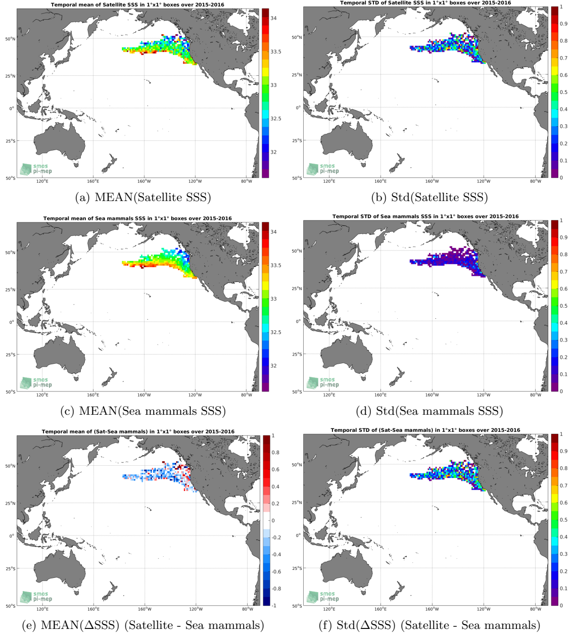
Figure 6: Temporal mean (left) and Std (right) of SSS from SMAP-L3-RSS-V3-8DAY-RUNNING-40KM (top), Sea mammals (middle), and of \Delta SSS (Satellite - Sea mammals). Only match-up pairs are used to generate these maps.
