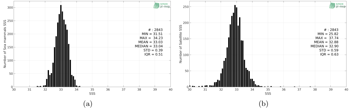
Figure 2: Histograms of SSS from Sea mammals (a) and SMAP-L3-RSS-V3-8DAY-RUNNING-40KM (b) considering all match-up pairs per bins of 0.1 over the Pacific Ocean Pi-MEP region and for the full satellite product period.
