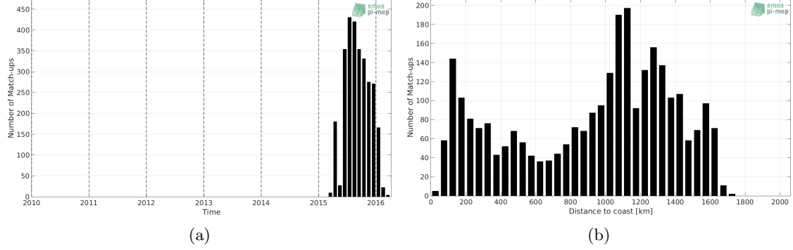
Figure 1: Number of match-ups between Sea mammals and SMAP-L3-RSS-V3-8DAY-RUNNING-40KM SSS as a function of time (a) and as function of the distance to coast (b) over the Pacific Ocean Pi-MEP region and for the full satellite product period.
