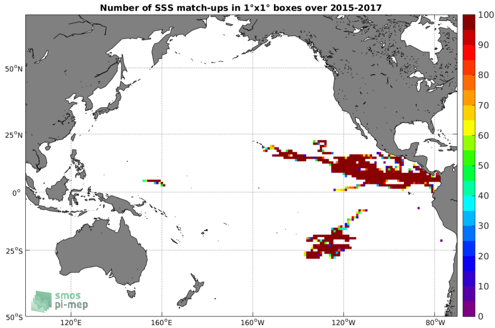
Figure 3: Number of SSS match-ups between Surface drifters SSS and the SMAP-L3-RSS-V3-8DAY-RUNNING-40KM SSS product for the Pacific Ocean Pi-MEP region over 1^{\circ} \times 1^{\circ} boxes and for the full satellite product period.
