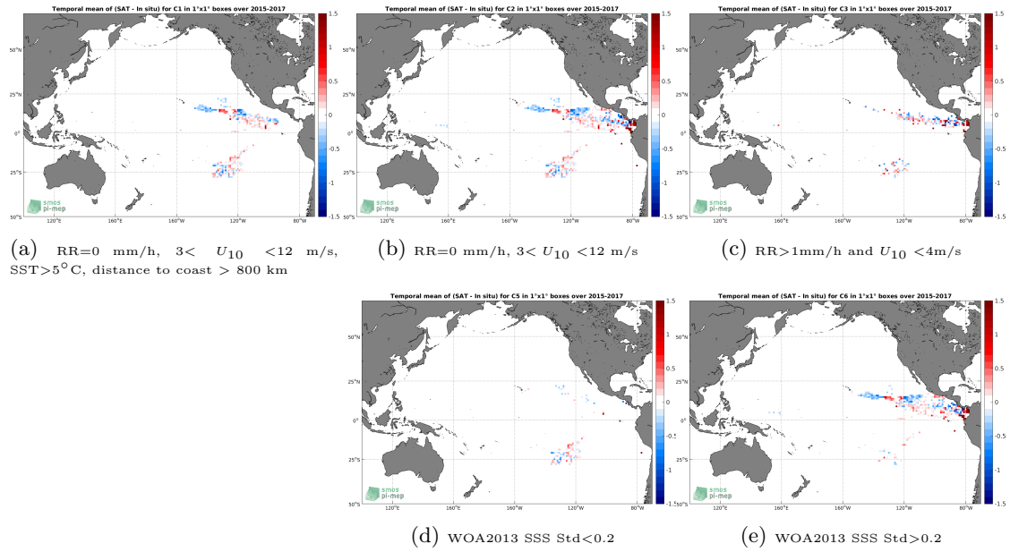
Figure 11: Temporal mean gridded over spatial boxes of size 1^\circ \times 1^\circ of \Delta SSS (SMAP-L3-RSS-V3-8DAY-RUNNING-40KM - Surface drifters) for 5 different subdatasets corresponding to:RR=0 mm/h, 3 < U_{10} < 12 m/s, SST >5^\circ C, distance to coast > 800 km (a), RR=0 mm/h, 3 < U_{10} < 12 m/s (b), RR >1 mm/h and U_{10} < 4 m/s (c), WOA2013 SSS Std <0.2 (d), WOA2013 SSS Std >0.2 (e).
