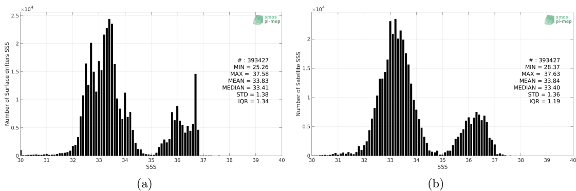
Figure 2: Histograms of SSS from Surface drifters (a) and SMAP-L3-RSS-V3-8DAY-RUNNING-40KM (b) considering all match-up pairs per bins of 0.1 over the Pacific Ocean Pi-MEP region and for the full satellite product period.
