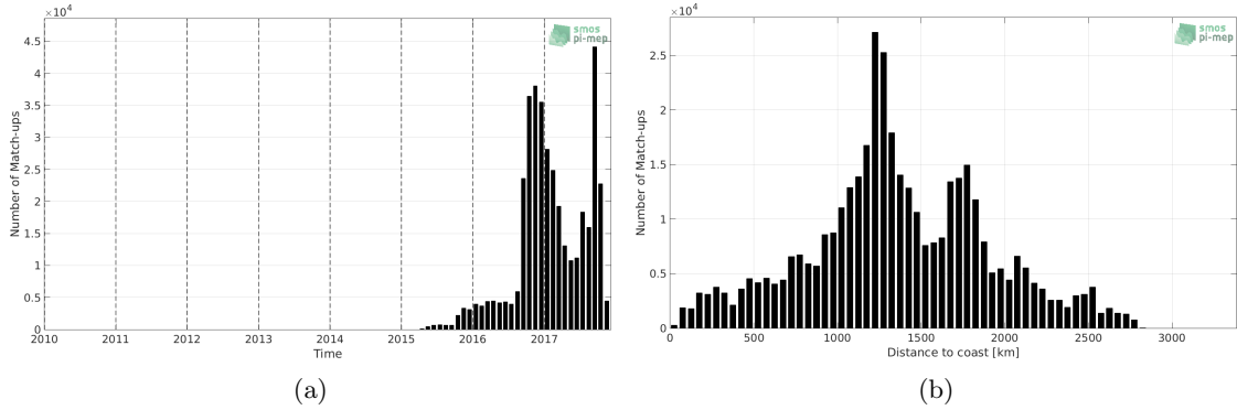
Figure 1: Number of match-ups between Surface drifters and SMAP-L3-RSS-V3-8DAY-RUNNING-40KM SSS as a function of time (a) and as function of the distance to coast (b) over the Pacific Ocean Pi-MEP region and for the full satellite product period.
