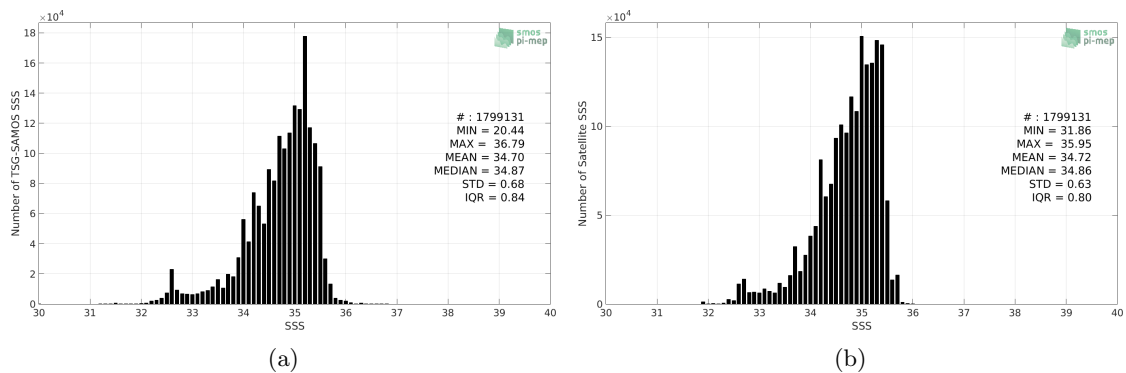
Figure 2: Histograms of SSS from TSG-SAMOS (a) and SMAP-L3-RSS-V3-MONTHLY-70KM (b) considering all match-up pairs per bins of 0.1 over the Pacific Ocean Pi-MEP region and for the full satellite product period.
