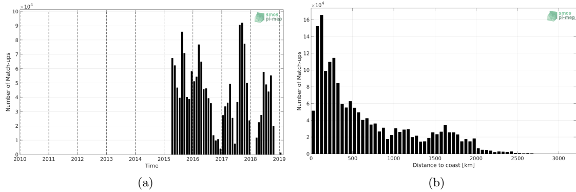
Figure 1: Number of match-ups between TSG-SAMOS and SMAP-L3-RSS-V3-MONTHLY-70KM SSS as a function of time (a) and as function of the distance to coast (b) over the Pacific Ocean Pi-MEP region and for the full satellite product period.
