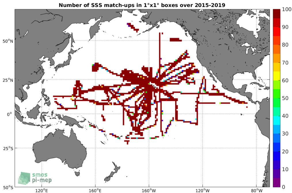
Figure 4: Number of SSS match-ups between TSG-SAMOS SSS and the SMAP-L3-RSS-V3-MONTHLY-70KM SSS product for the Pacific Ocean Pi-MEP region over 1^\circ \times 1^\circ boxes and for the full satellite product period.
