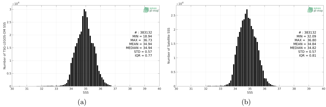
Figure 2: Histograms of SSS from TSG-LEGOS-DM (a) and SMAP-L3-RSS-V3-MONTHLY-70KM (b) considering all match-up pairs per bins of 0.1 over the Pacific Ocean Pi-MEP region and for the full satellite product period.
