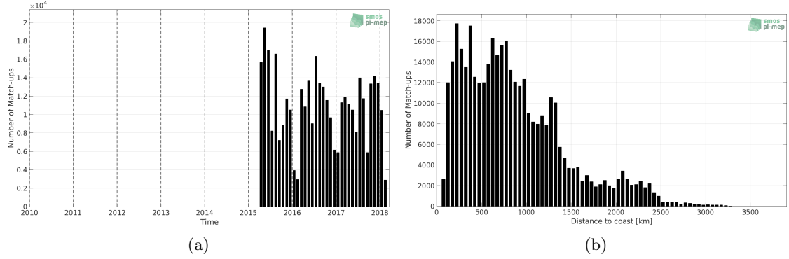
Figure 1: Number of match-ups between TSG-LEGOS-DM and SMAP-L3-RSS-V3-MONTHLY-70KM SSS as a function of time (a) and as function of the distance to coast (b) over the Pacific Ocean Pi-MEP region and for the full satellite product period.
