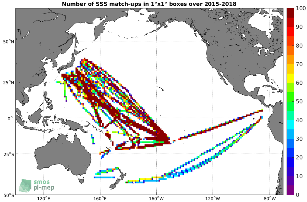
Figure 4: Number of SSS match-ups between TSG-LEGOS-DM SSS and the SMAP-L3-RSS-V3-MONTHLY-70KM SSS product for the Pacific Ocean Pi-MEP region over 1^\circ \times 1^\circ boxes and for the full satellite product period.
