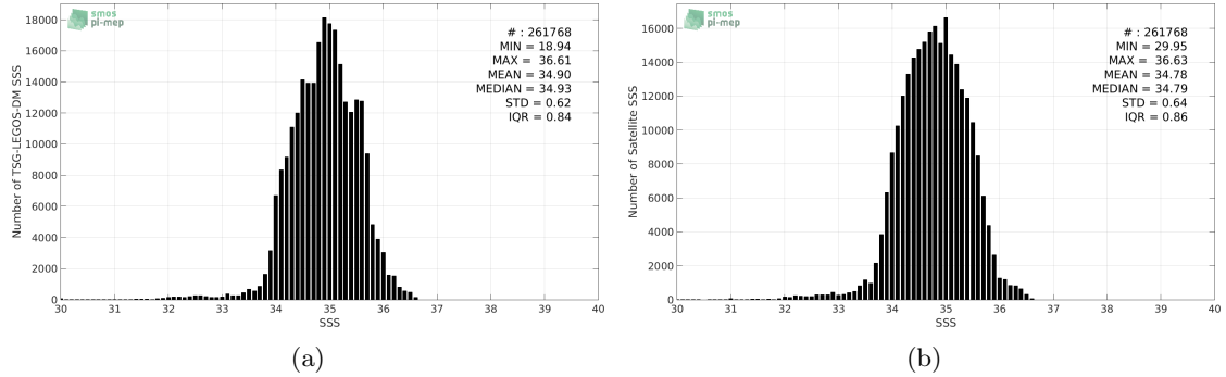
Figure 2: Histograms of SSS from TSG-LEGOS-DM (a) and SMAP-L3-RSS-V3-MONTHLY-70KM (b) considering all match-up pairs per bins of 0.1 over the Pacific Ocean Pi-MEP region and for the full satellite product period.
