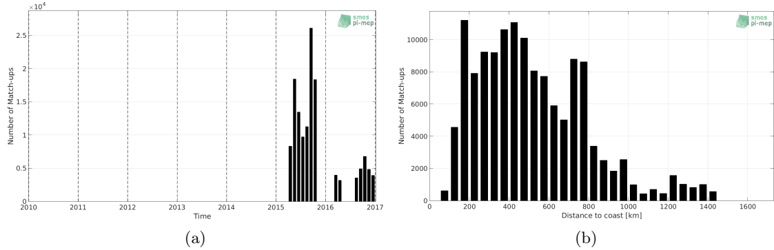
Figure 1: Number of match-ups between TSG-GOSUD-Research-vessel and SMAP-L3-RSS-V3-MONTHLY-70KM SSS as a function of time (a) and as function of the distance to coast (b) over the Pacific Ocean Pi-MEP region and for the full satellite product period.
