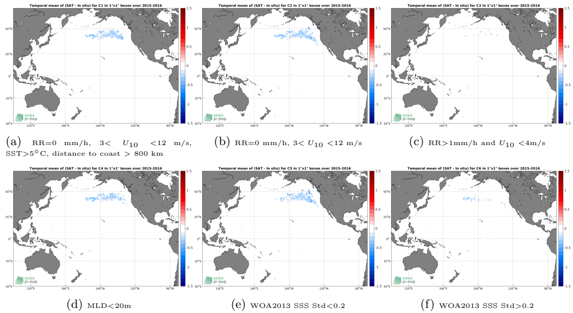
Figure 12: Temporal mean gridded over spatial boxes of size 1^\circ \times 1^\circ of \Delta SSS (SMAP-L3-RSS-V3-MONTHLY-70KM - Sea mammals) for 6 different subdatasets corresponding to:RR=0 mm/h, 3 < U_{10} < 12 m/s, SST >5^\circ C, distance to coast > 800 km (a), RR=0 mm/h, 3 < U_{10} < 12 m/s (b), RR >1 mm/h and U_{10} < 4 m/s (c),MLD <20 m (d),WOA2013 SSS Std <0.2 (e),WOA2013 SSS Std >0.2 (f).
