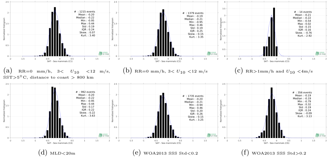
Figure 13: Normalized histogram of \Delta\text{SSS} (SMAP-L3-RSS-V3-MONTHLY-70KM - Sea mammals) for 6 different subdatasets corresponding to: RR=0 mm/h, 3 < U_{10} < 12 m/s, SST>5°C, distance to coast > 800 km (a), RR=0 mm/h, 3 < U_{10} < 12 m/s (b), RR>1mm/h and U_{10} < 4 m/s (c), MLD<20m (d), WOA2013 SSS Std<0.2 (e), WOA2013 SSS Std>0.2 (f).
