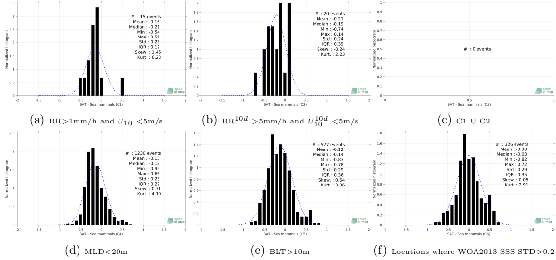
Figure 13: Normalized histogram of \Delta SSS (SMAP-L3-RSS-V3-MONTHLY-70KM - Sea mammals) for 6 different subdatasets corresponding to: RR > 1\text{mm/h} and U_{10} < 5\text{m/s} (a), RR^{10d} > 5\text{mm/h} and U_{10}^{10d} < 5\text{m/s} (b), C1 U C2 (c), MLD < 20\text{m} (d), BLT > 10\text{m} (e), Locations where WOA2013 SSS STD > 0.2 (f).
