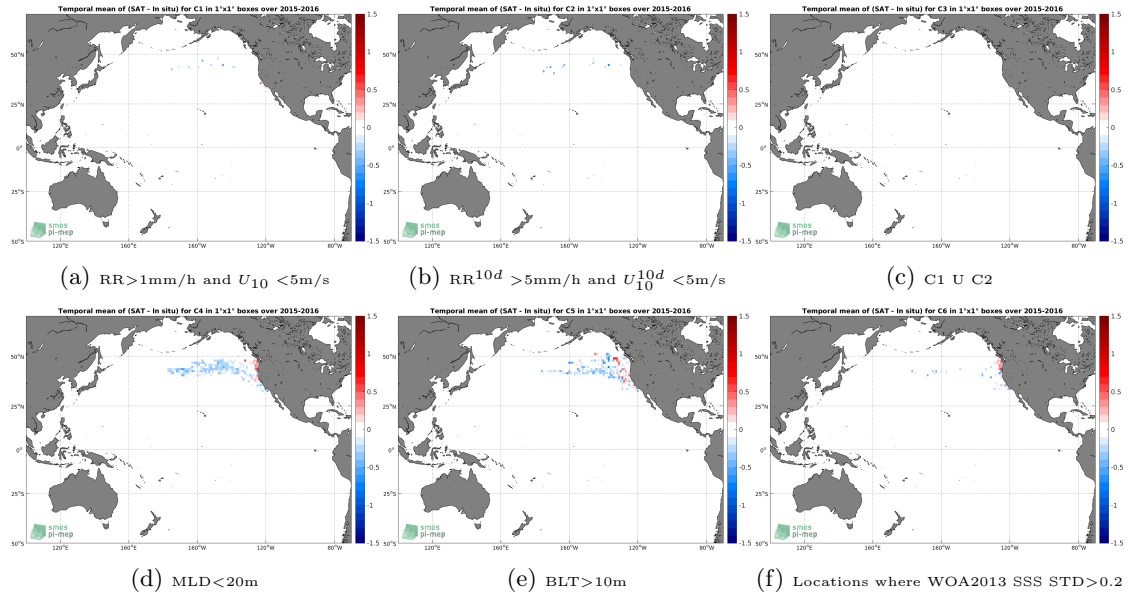
Figure 12: Temporal mean gridded over spatial boxes of size 1^\circ \times 1^\circ of \Delta\text{SSS} (SMAP-L3-RSS-V3-MONTHLY-70KM - Sea mammals) for 6 different subdatasets corresponding to: RR > 1\text{mm/h} and U_{10} < 5\text{m/s} (a), RR^{10d} > 5\text{mm/h} and U_{10}^{10d} < 5\text{m/s} (b), C1 U C2 (c), MLD < 20\text{m} (d), BLT > 10\text{m} (e), Locations where WOA2013 SSS STD > 0.2 (f).
