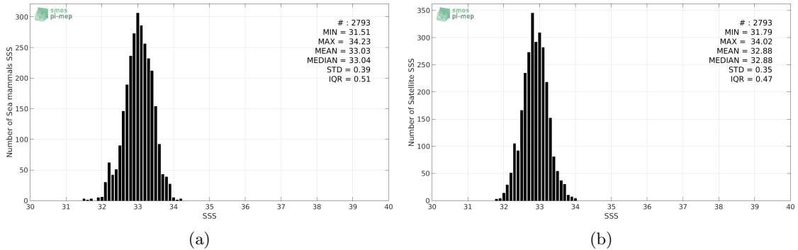
Figure 2: Histograms of SSS from Sea mammals (a) and SMAP-L3-RSS-V3-MONTHLY-70KM (b) considering all match-up pairs per bins of 0.1 over the Pacific Ocean Pi-MEP region and for the full satellite product period.
