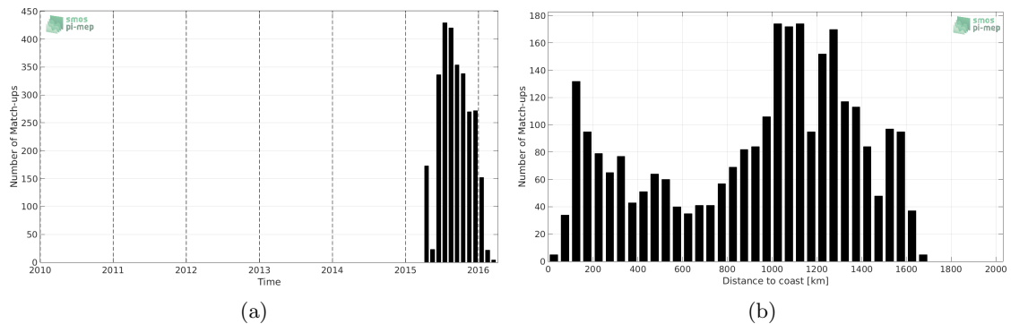
Figure 1: Number of match-ups between Sea mammals and SMAP-L3-RSS-V3-MONTHLY-70KM SSS as a function of time (a) and as function of the distance to coast (b) over the Pacific Ocean Pi-MEP region and for the full satellite product period.
