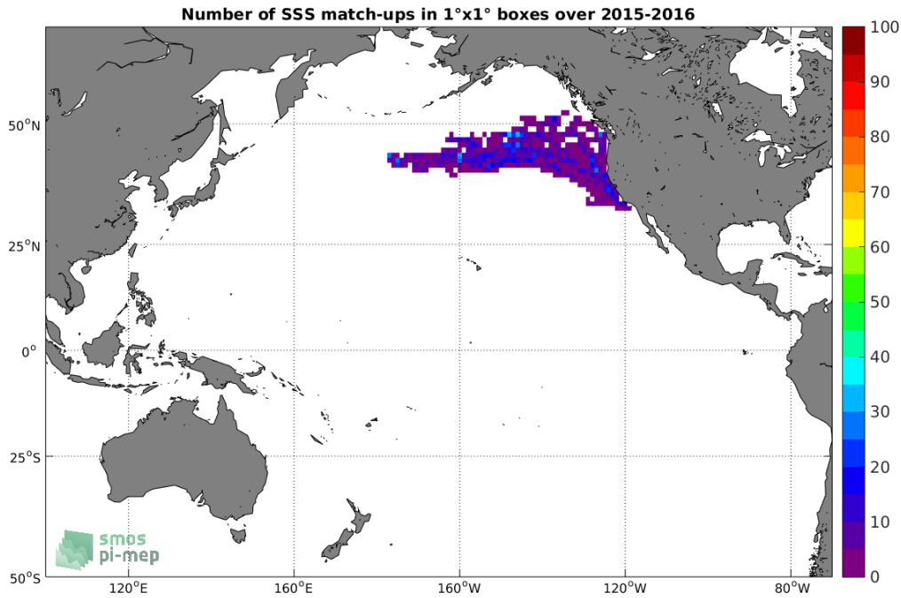
Figure 4: Number of SSS match-ups between Sea mammals SSS and the SMAP-L3-RSS-V3-MONTHLY-70KM SSS product for the Pacific Ocean Pi-MEP region over 1^\circ \times 1^\circ boxes and for the full satellite product period.
