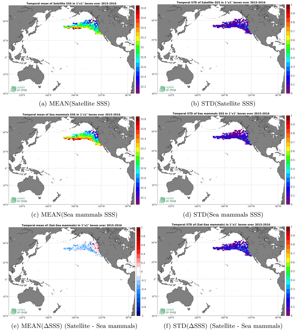
Figure 6: Temporal mean (left) and STD (right) of SSS from SMAP-L3-RSS-V3-MONTHLY-70KM (top), Sea mammals (middle), and of \Delta SSS (Satellite - Sea mammals). Only match-up pairs are used to generate these maps.
