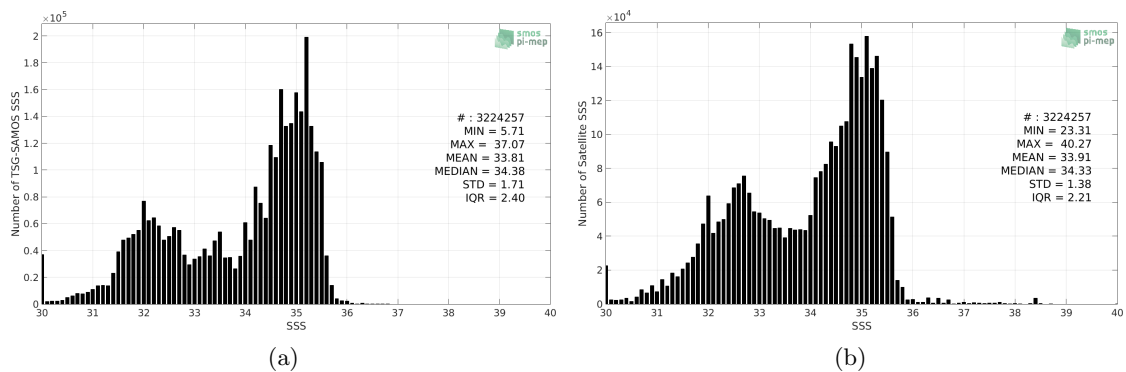
Figure 2: Histograms of SSS from TSG-SAMOS (a) and SMAP-L3-RSS-V3-MONTHLY-0.25DEG-40KM (b) considering all match-up pairs per bins of 0.1 over the Pacific Ocean Pi-MEP region and for the full satellite product period.
