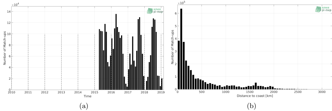
Figure 1: Number of match-ups between TSG-SAMOS and SMAP-L3-RSS-V3-MONTHLY-0.25DEG-40KM SSS as a function of time (a) and as function of the distance to coast (b) over the Pacific Ocean Pi-MEP region and for the full satellite product period.
