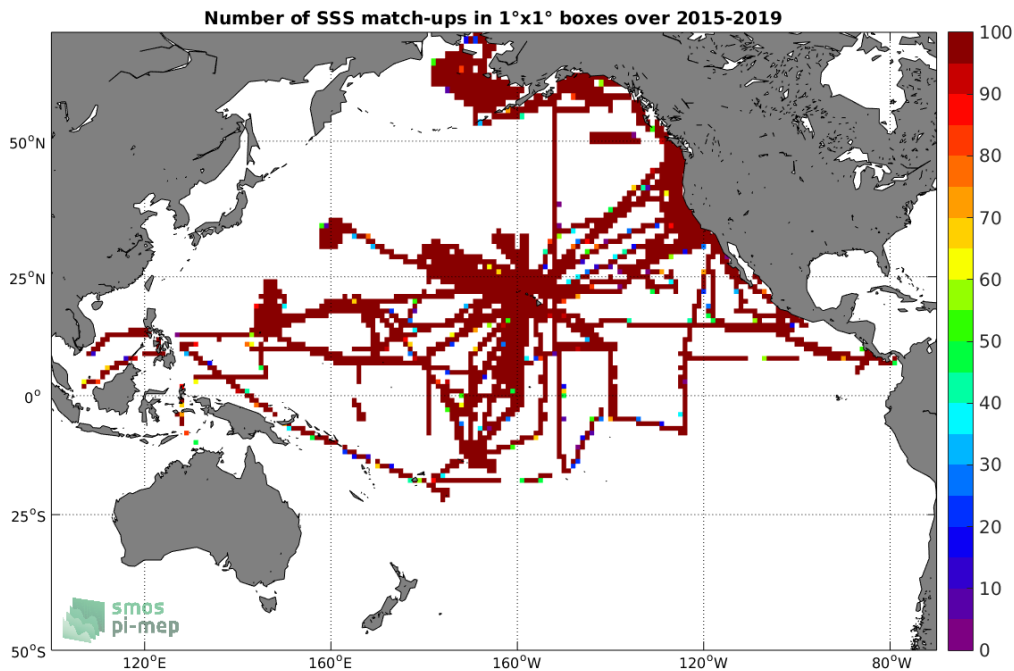
Figure 4: Number of SSS match-ups between TSG-SAMOS SSS and the SMAP-L3-RSS-V3-MONTHLY-0.25DEG-40KM SSS product for the Pacific Ocean Pi-MEP region over 1^\circ \times 1^\circ boxes and for the full satellite product period.
