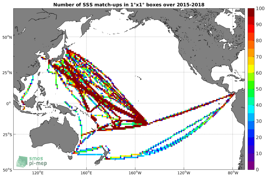
Figure 4: Number of SSS match-ups between TSG-LEGOS-DM SSS and the SMAP-L3-RSS-V3-MONTHLY-0.25DEG-40KM SSS product for the Pacific Ocean Pi-MEP region over 1^\circ \times 1^\circ boxes and for the full satellite product period.
