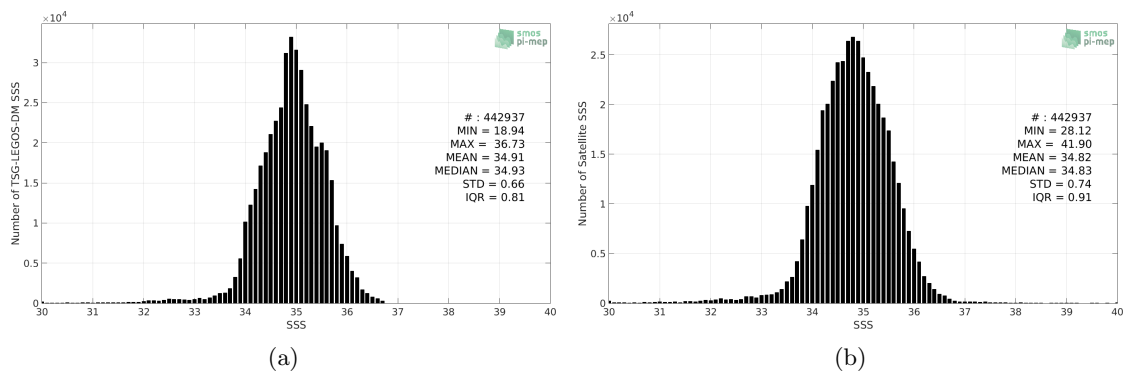
Figure 2: Histograms of SSS from TSG-LEGOS-DM (a) and SMAP-L3-RSS-V3-MONTHLY-0.25DEG-40KM (b) considering all match-up pairs per bins of 0.1 over the Pacific Ocean Pi-MEP region and for the full satellite product period.
