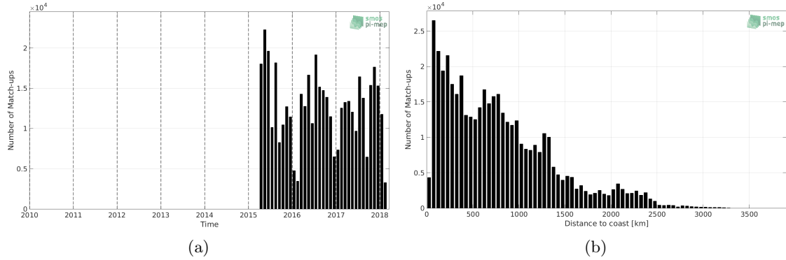
Figure 1: Number of match-ups between TSG-LEGOS-DM and SMAP-L3-RSS-V3-MONTHLY-0.25DEG-40KM SSS as a function of time (a) and as function of the distance to coast (b) over the Pacific Ocean Pi-MEP region and for the full satellite product period.
