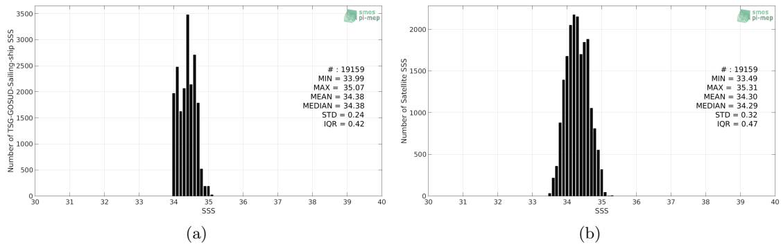
Figure 2: Histograms of SSS from TSG-GOSUD-Sailing-ship (a) and SMAP-L3-RSS-V3-MONTHLY-0.25DEG-40KM (b) considering all match-up pairs per bins of 0.1 over the Pacific Ocean Pi-MEP region and for the full satellite product period.
