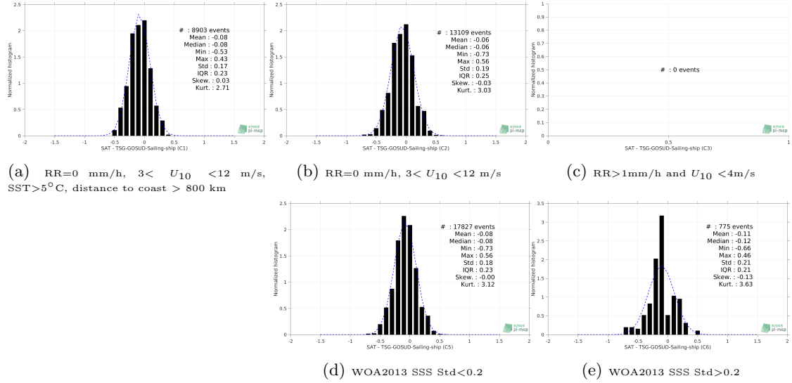
Figure 13: Normalized histogram of \Delta\text{SSS} (SMAP-L3-RSS-V3-MONTHLY-0.25DEG-40KM - TSG-GOSUD-Sailing-ship) for 5 different subdatasets corresponding to: RR=0 mm/h, 3 < U_{10} < 12 m/s, SST > 5^\circ\text{C} , distance to coast > 800 km (a), RR=0 mm/h, 3 < U_{10} < 12 m/s (b), RR > 1 mm/h and U_{10} < 4 m/s (c), WOA2013 SSS Std < 0.2 (d), WOA2013 SSS Std > 0.2 (e).
