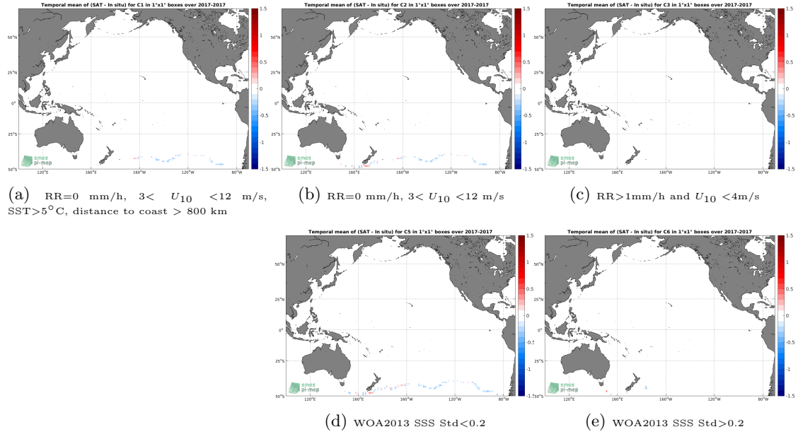
Figure 12: Temporal mean gridded over spatial boxes of size 1^\circ \times 1^\circ of \Delta SSS (SMAP-L3-RSS-V3-MONTHLY-0.25DEG-40KM - TSG-GOSUD-Sailing-ship) for 5 different subdatasets corresponding to:RR=0 mm/h, 3 < U_{10} < 12 m/s, SST >5^\circ C, distance to coast > 800 km (a), RR=0 mm/h, 3 < U_{10} < 12 m/s (b), RR >1 mm/h and U_{10} < 4 m/s (c), WOA2013 SSS Std <0.2 (d), WOA2013 SSS Std >0.2 (e).
