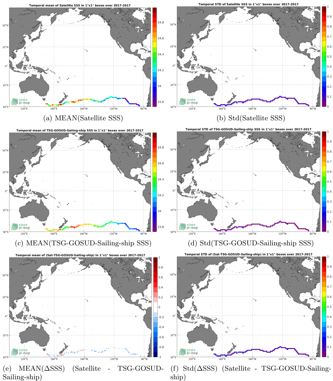
Figure 6: Temporal mean (left) and Std (right) of SSS from SMAP-L3-RSS-V3-MONTHLY-0.25DEG-40KM (top), TSG-GOSUD-Sailing-ship (middle), and of \Delta SSS (Satellite - TSG-GOSUD-Sailing-ship). Only match-up pairs are used to generate these maps.
