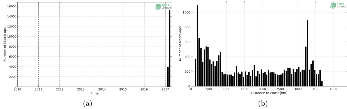
Figure 1: Number of match-ups between TSG-GOSUD-Sailing-ship and SMAP-L3-RSS-V3-MONTHLY-0.25DEG-40KM SSS as a function of time (a) and as function of the distance to coast (b) over the Pacific Ocean Pi-MEP region and for the full satellite product period.
