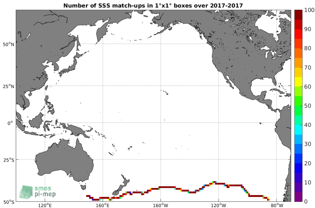
Figure 4: Number of SSS match-ups between TSG-GOSUD-Sailing-ship SSS and the SMAP-L3-RSS-V3-MONTHLY-0.25DEG-40KM SSS product for the Pacific Ocean Pi-MEP region over 1^\circ \times 1^\circ boxes and for the full satellite product period.
