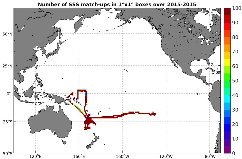
Figure 4: Number of SSS match-ups between TSG-GOSUD-Research-vessel SSS and the SMAP-L3-RSS-V2-8DAY-RUNNING-40KM SSS product for the Pacific Ocean Pi-MEP region over 1^\circ \times 1^\circ boxes and for the full satellite product period.
