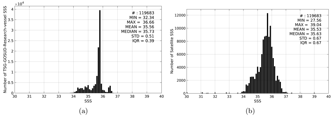
Figure 2: Histograms of SSS from TSG-GOSUD-Research-vessel (a) and SMAP-L3-RSS-V2-8DAY-RUNNING-40KM (b) considering all match-up pairs per bins of 0.1 over the Pacific Ocean Pi-MEP region and for the full satellite product period.
