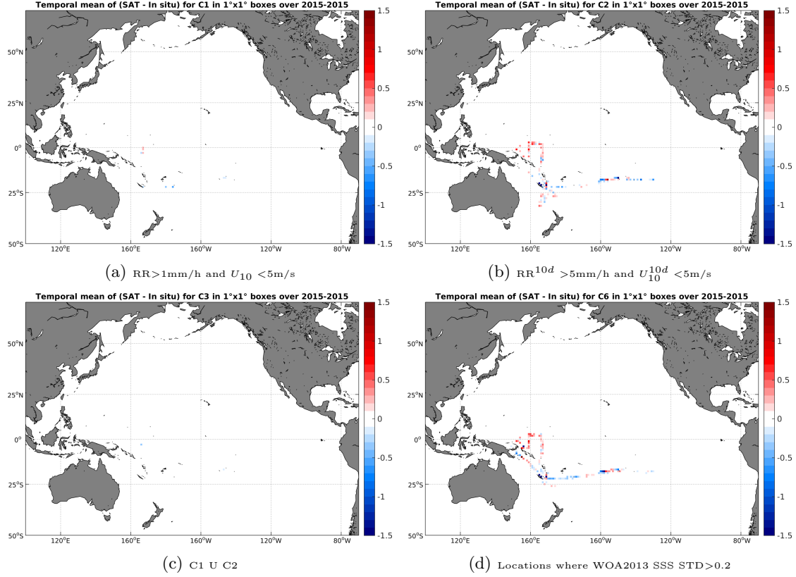
Figure 12: Temporal mean gridded over spatial boxes of size 1^\circ \times 1^\circ of \Delta SSS (SMAP-L3-RSS-V2-8DAY-RUNNING-40KM - TSG-GOSUD-Research-vessel) for 4 different subdatasets corresponding to: RR > 1mm/h and U_{10} < 5 m/s (a), RR^{10d} > 5 mm/h and U_{10}^{10d} < 5 m/s (b), C1 U C2 (c), Locations where WOA2013 SSS STD > 0.2 (d).
