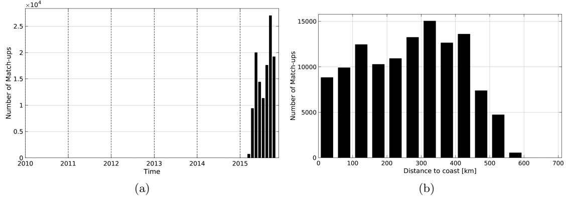
Figure 1: Number of match-ups between TSG-GOSUD-Research-vessel and SMAP-L3-RSS-V2-8DAY-RUNNING-40KM SSS as a function of time (a) and as function of the distance to coast (b) over the Pacific Ocean Pi-MEP region and for the full satellite product period.
