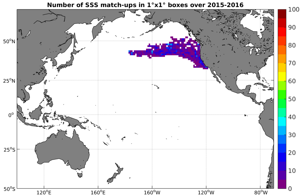
Figure 4: Number of SSS match-ups between Sea mammals SSS and the SMAP-L3-RSS-V2-8DAY-RUNNING-40KM SSS product for the Pacific Ocean Pi-MEP region over 1^\circ \times 1^\circ boxes and for the full satellite product period.
