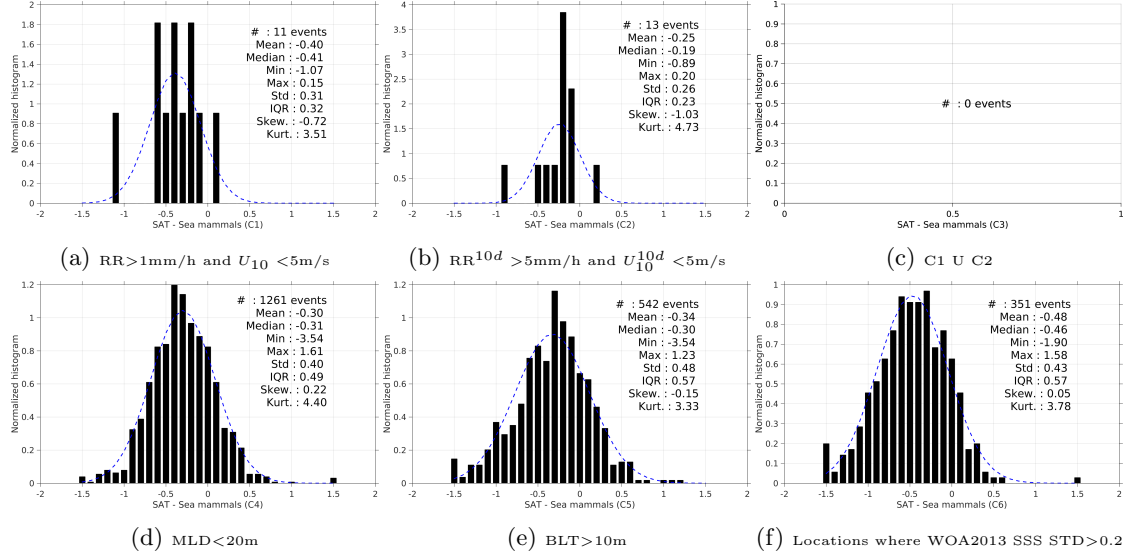
Figure 13: Normalized histogram of \Delta SSS (SMAP-L3-RSS-V2-8DAY-RUNNING-40KM - Sea mammals) for 6 different subdatasets corresponding to: RR > 1\text{mm/h} and U_{10} < 5\text{m/s} (a), RR^{10d} > 5\text{mm/h} and U_{10}^{10d} < 5\text{m/s} (b), C1 \cup C2 (c), MLD < 20\text{m} (d), BLT > 10\text{m} (e), Locations where WOA2013 SSS STD > 0.2 (f).
