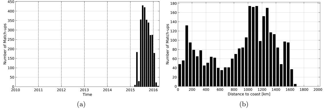
Figure 1: Number of match-ups between Sea mammals and SMAP-L3-RSS-V2-8DAY-RUNNING-40KM SSS as a function of time (a) and as function of the distance to coast (b) over the Pacific Ocean Pi-MEP region and for the full satellite product period.
