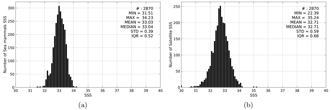
Figure 2: Histograms of SSS from Sea mammals (a) and SMAP-L3-RSS-V2-8DAY-RUNNING-40KM (b) considering all match-up pairs per bins of 0.1 over the Pacific Ocean Pi-MEP region and for the full satellite product period.
