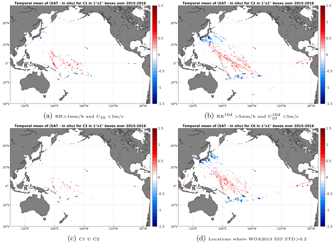
Figure 12: Temporal mean gridded over spatial boxes of size 1^\circ \times 1^\circ of \Delta SSS (SMAP-L3-RSS-V2-8DAY-RUNNING-70KM - TSG-LEGOS-DM) for 4 different subdatasets corresponding to: RR > 1mm/h and U_{10} < 5\text{m/s} (a), RR^{10d} > 5\text{mm/h} and U_{10}^{10d} < 5\text{m/s} (b), C1 U C2 (c), Locations where WOA2013 SSS STD > 0.2 (d).
