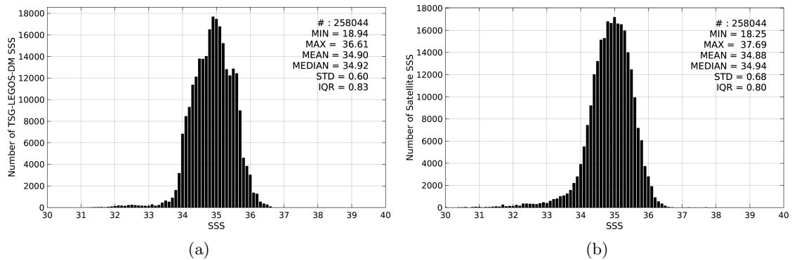
Figure 2: Histograms of SSS from TSG-LEGOS-DM (a) and SMAP-L3-RSS-V2-8DAY-RUNNING-70KM (b) considering all match-up pairs per bins of 0.1 over the Pacific Ocean Pi-MEP region and for the full satellite product period.
