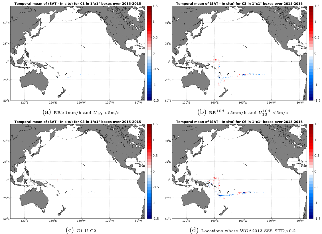
Figure 12: Temporal mean gridded over spatial boxes of size 1^\circ \times 1^\circ of \Delta SSS (SMAP-L3-RSS-V2-8DAY-RUNNING-70KM - TSG-GOSUD-Research-vessel) for 4 different subdatasets corresponding to: RR > 1\text{mm/h} and U_{10} < 5\text{m/s} (a), RR^{10d} > 5\text{mm/h} and U_{10}^{10d} < 5\text{m/s} (b), C1 U C2 (c), Locations where WOA2013 SSS STD > 0.2 (d).
