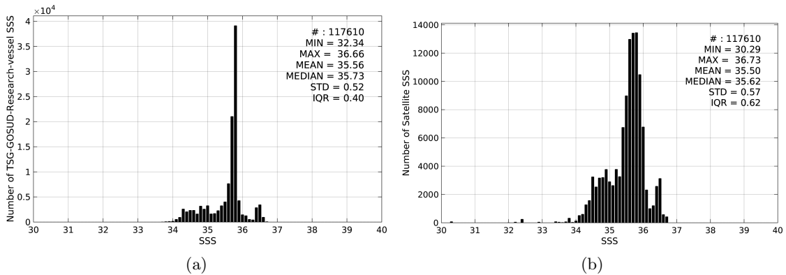
Figure 2: Histograms of SSS from TSG-GOSUD-Research-vessel (a) and SMAP-L3-RSS-V2-8DAY-RUNNING-70KM (b) considering all match-up pairs per bins of 0.1 over the Pacific Ocean Pi-MEP region and for the full satellite product period.
