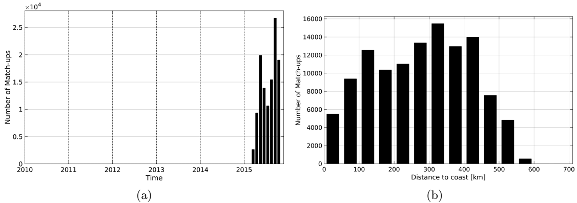
Figure 1: Number of match-ups between TSG-GOSUD-Research-vessel and SMAP-L3-RSS-V2-8DAY-RUNNING-70KM SSS as a function of time (a) and as function of the distance to coast (b) over the Pacific Ocean Pi-MEP region and for the full satellite product period.
