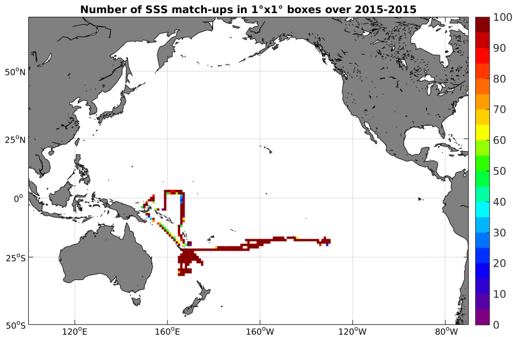
Figure 4: Number of SSS match-ups between TSG-GOSUD-Research-vessel SSS and the SMAP-L3-RSS-V2-8DAY-RUNNING-70KM SSS product for the Pacific Ocean Pi-MEP region over 1°x1° boxes and for the full satellite product period.
