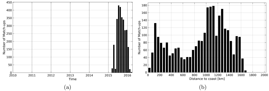
Figure 1: Number of match-ups between Sea mammals and SMAP-L3-RSS-V2-8DAY-RUNNING-70KM SSS as a function of time (a) and as function of the distance to coast (b) over the Pacific Ocean Pi-MEP region and for the full satellite product period.
