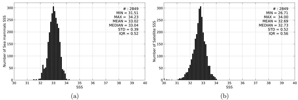
Figure 2: Histograms of SSS from Sea mammals (a) and SMAP-L3-RSS-V2-8DAY-RUNNING-70KM (b) considering all match-up pairs per bins of 0.1 over the Pacific Ocean Pi-MEP region and for the full satellite product period.
