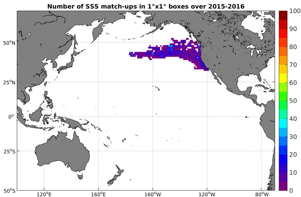
Figure 4: Number of SSS match-ups between Sea mammals SSS and the SMAP-L3-RSS-V2-8DAY-RUNNING-70KM SSS product for the Pacific Ocean Pi-MEP region over 1°x1° boxes and for the full satellite product period.
