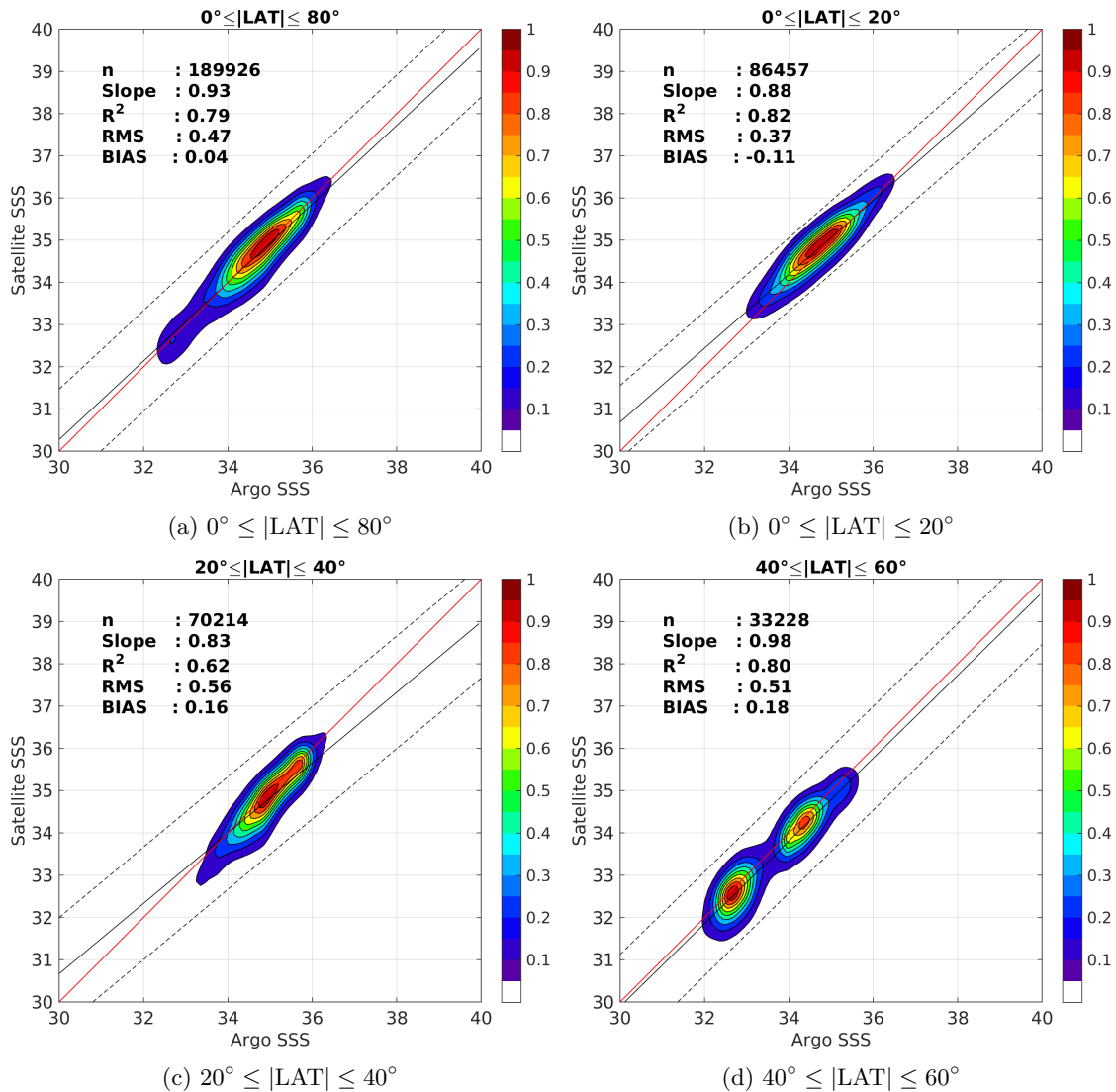
Figure 9: Contour maps of the concentration of SMAP-L3-RSS-V2-8DAY-RUNNING-70KM SSS (y-axis) versus Argo SSS (x-axis) at match-up pairs for different latitude bands. For each plot, the red line shows x=y . The black thin and dashed lines indicate a linear fit through the data cloud and the \pm 95\% confidence levels, respectively. The number match-up pairs n , the slope and R^2 coefficient of the linear fit, the root mean square (RMS) and the mean bias between satellite and in situ data are indicated for each latitude band in each plots.
