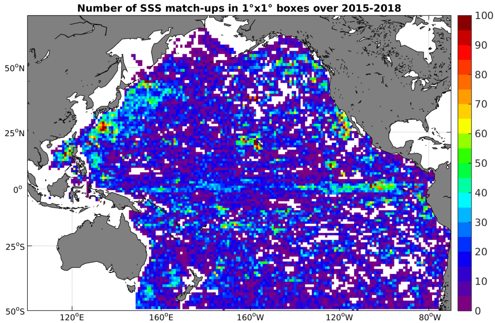
Figure 4: Number of SSS match-ups between Argo SSS and the SMAP-L3-RSS-V2-8DAY-RUNNING-70KM SSS product for the Pacific Ocean Pi-MEP region over 1^\circ \times 1^\circ boxes and for the full satellite product period.
