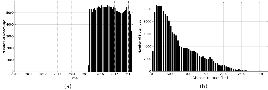
Figure 1: Number of match-ups between Argo and SMAP-L3-RSS-V2-8DAY-RUNNING-70KM SSS as a function of time (a) and as function of the distance to coast (b) over the Pacific Ocean Pi-MEP region and for the full satellite product period.
