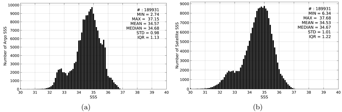
Figure 2: Histograms of SSS from Argo (a) and SMAP-L3-RSS-V2-8DAY-RUNNING-70KM (b) considering all match-up pairs per bins of 0.1 over the Pacific Ocean Pi-MEP region and for the full satellite product period.
