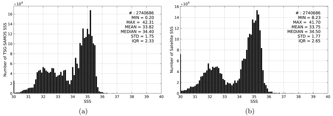
Figure 2: Histograms of SSS from TSG-SAMOS (a) and SMAP-L3-RSS-V2-MONTHLY-0.25DEG-40KM (b) considering all match-up pairs per bins of 0.1 over the Pacific Ocean Pi-MEP region and for the full satellite product period.
