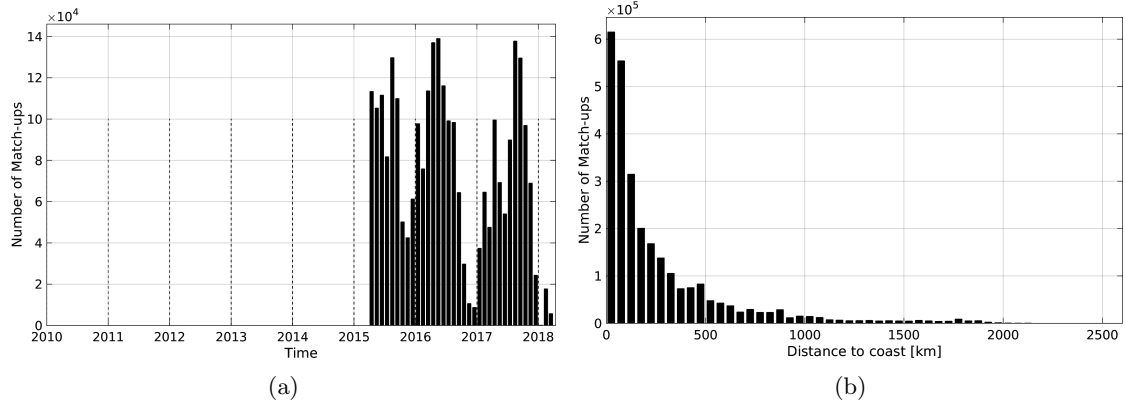
Figure 1: Number of match-ups between TSG-SAMOS and SMAP-L3-RSS-V2-MONTHLY-0.25DEG-40KM SSS as a function of time (a) and as function of the distance to coast (b) over the Pacific Ocean Pi-MEP region and for the full satellite product period.
