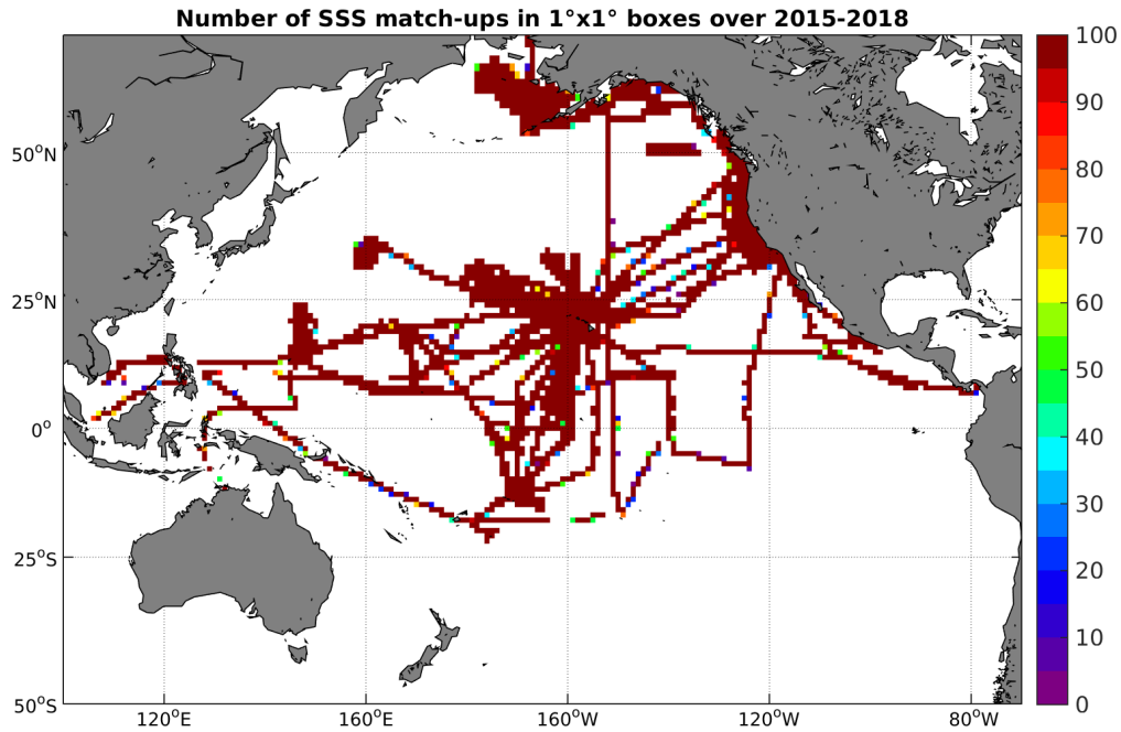
Figure 4: Number of SSS match-ups between TSG-SAMOS SSS and the SMAP-L3-RSS-V2-MONTHLY-0.25DEG-40KM SSS product for the Pacific Ocean Pi-MEP region over 1^\circ \times 1^\circ boxes and for the full satellite product period.
