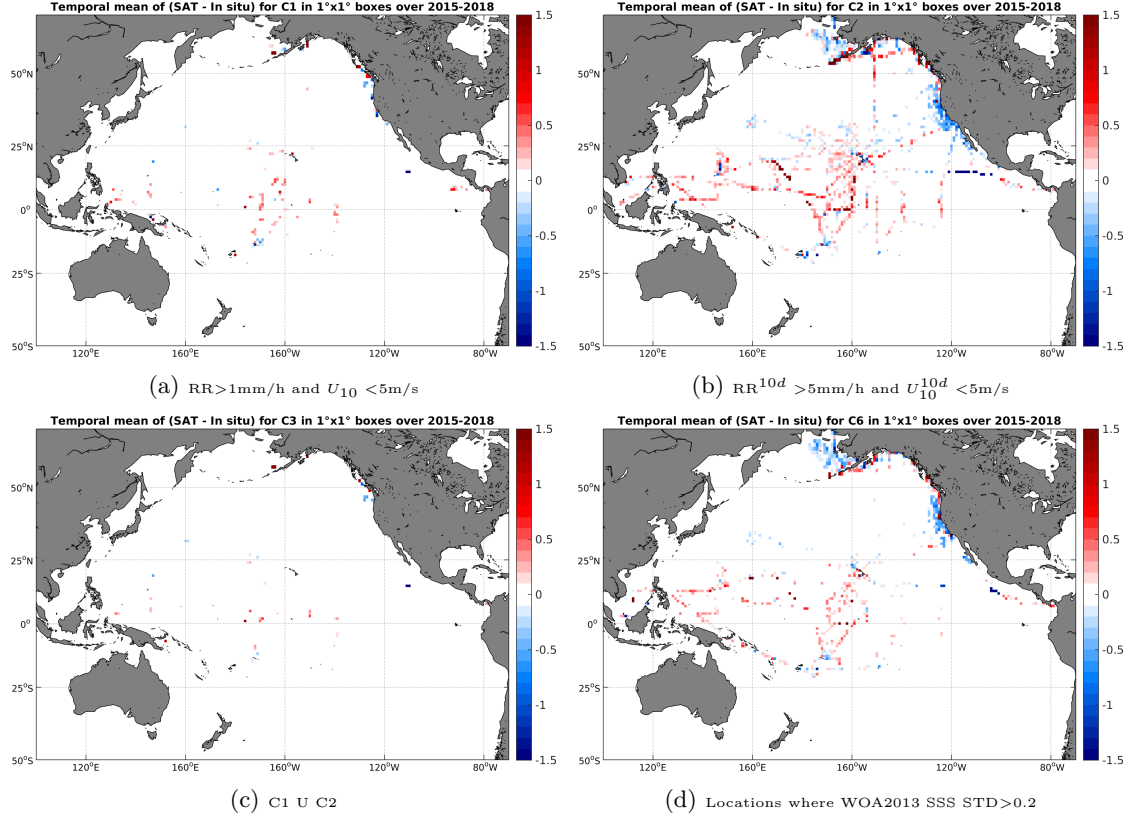
Figure 12: Temporal mean gridded over spatial boxes of size 1^\circ \times 1^\circ of \Delta SSS (SMAP-L3-RSS-V2-MONTHLY-0.25DEG-40KM - TSG-SAMOS) for 4 different subdatasets corresponding to: RR > 1mm/h and U_{10} < 5 m/s (a), RR^{10d} > 5 mm/h and U_{10}^{10d} < 5 m/s (b), C1 U C2 (c), Locations where WOA2013 SSS STD > 0.2 (d).
