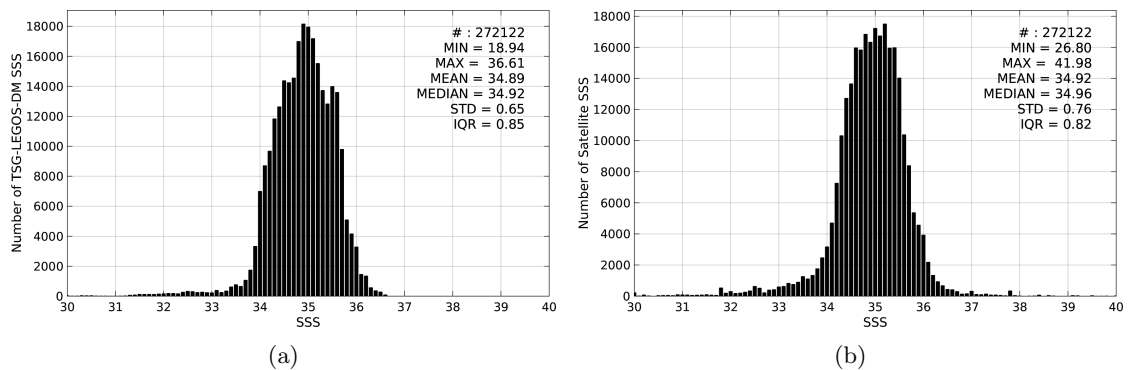
Figure 2: Histograms of SSS from TSG-LEGOS-DM (a) and SMAP-L3-RSS-V2-MONTHLY-0.25DEG-40KM (b) considering all match-up pairs per bins of 0.1 over the Pacific Ocean Pi-MEP region and for the full satellite product period.
