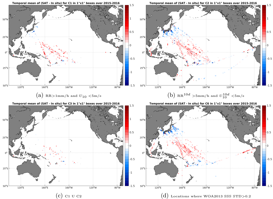
Figure 12: Temporal mean gridded over spatial boxes of size 1^\circ \times 1^\circ of \Delta SSS (SMAP-L3-RSS-V2-MONTHLY-0.25DEG-40KM - TSG-LEGOS-DM) for 4 different subdatasets corresponding to: RR > 1 mm/h and U_{10} < 5 m/s (a), RR 10d > 5 mm/h and U_{10}^{10d} < 5 m/s (b), C1 U C2 (c), Locations where WOA2013 SSS STD > 0.2 (d).
