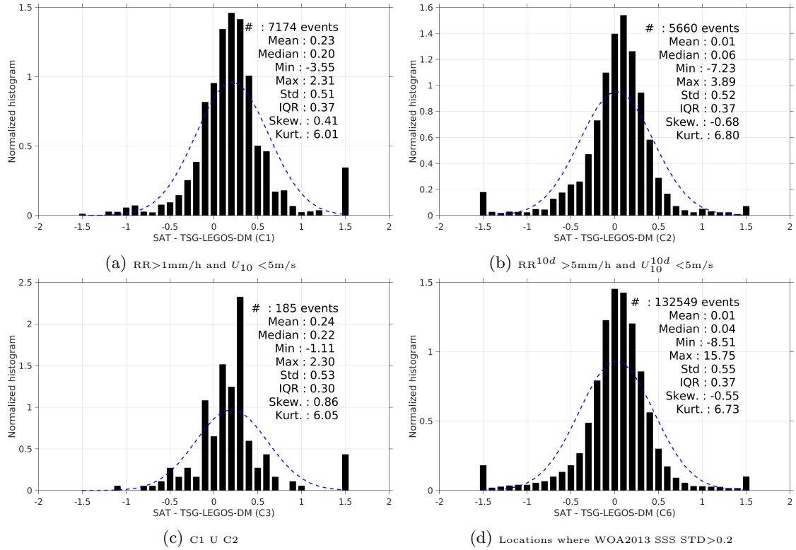
Figure 13: Normalized histogram of \Delta\text{SSS} (SMAP-L3-RSS-V2-MONTHLY-0.25DEG-40KM - TSG-LEGOS-DM) for 6 different subdatasets corresponding to: RR > 1mm/h and U_{10} < 5\text{m/s} (a), RR^{10d} > 5\text{mm/h} and U_{10}^{10d} < 5\text{m/s} (b), C1 U C2 (c), Locations where WOA2013 SSS STD > 0.2 (d).
