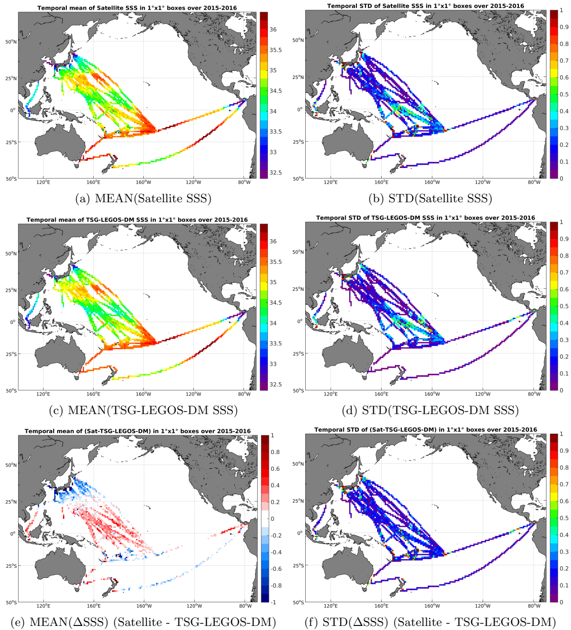
Figure 6: Temporal mean (left) and STD (right) of SSS from SMAP-L3-RSS-V2-MONTHLY-0.25DEG-40KM (top), TSG-LEGOS-DM (middle), and of \Delta SSS (Satellite - TSG-LEGOS-DM). Only match-up pairs are used to generate these maps.
