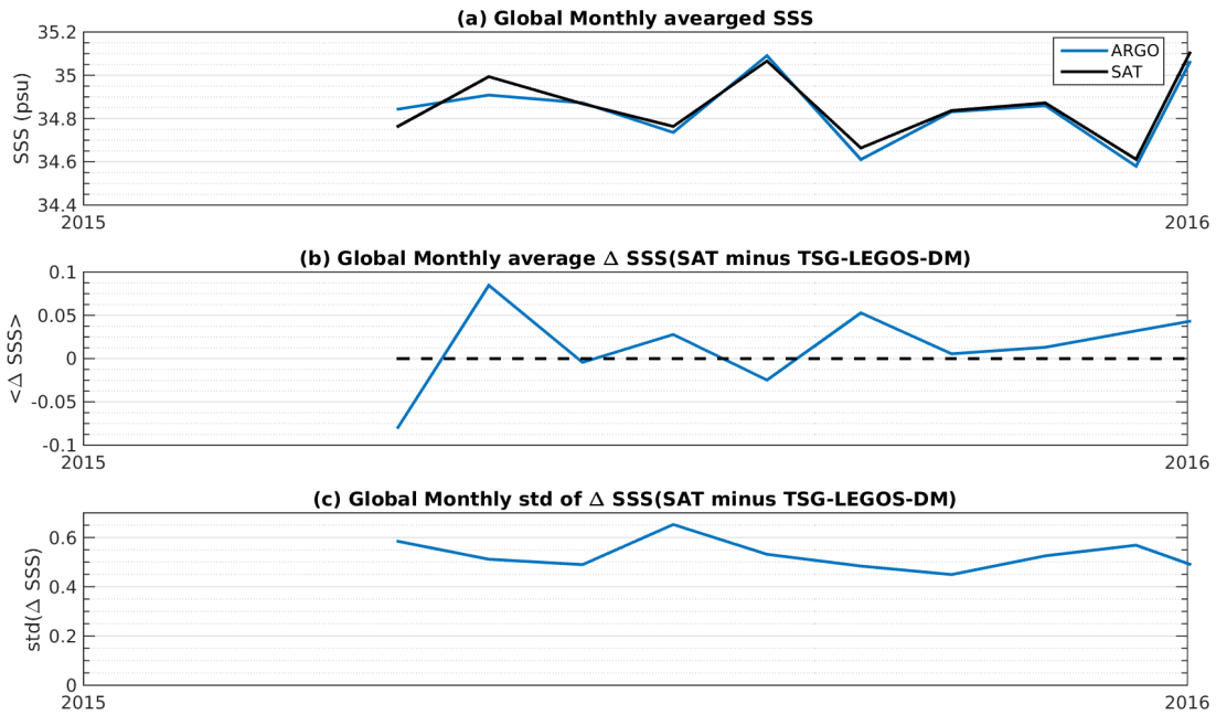
Figure 7: Time series of the monthly averaged mean SSS (top), mean \Delta SSS (Satellite - TSG-LEGOS-DM) and STD of \Delta SSS (Satellite - TSG-LEGOS-DM) over the Pacific Ocean Pi-MEP region considering all match-ups collected by the Pi-MEP platform.
