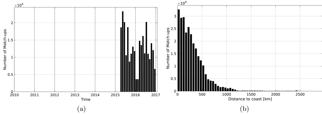
Figure 1: Number of match-ups between TSG-LEGOS-DM and SMAP-L3-RSS-V2-MONTHLY-0.25DEG-40KM SSS as a function of time (a) and as function of the distance to coast (b) over the Pacific Ocean Pi-MEP region and for the full satellite product period.
