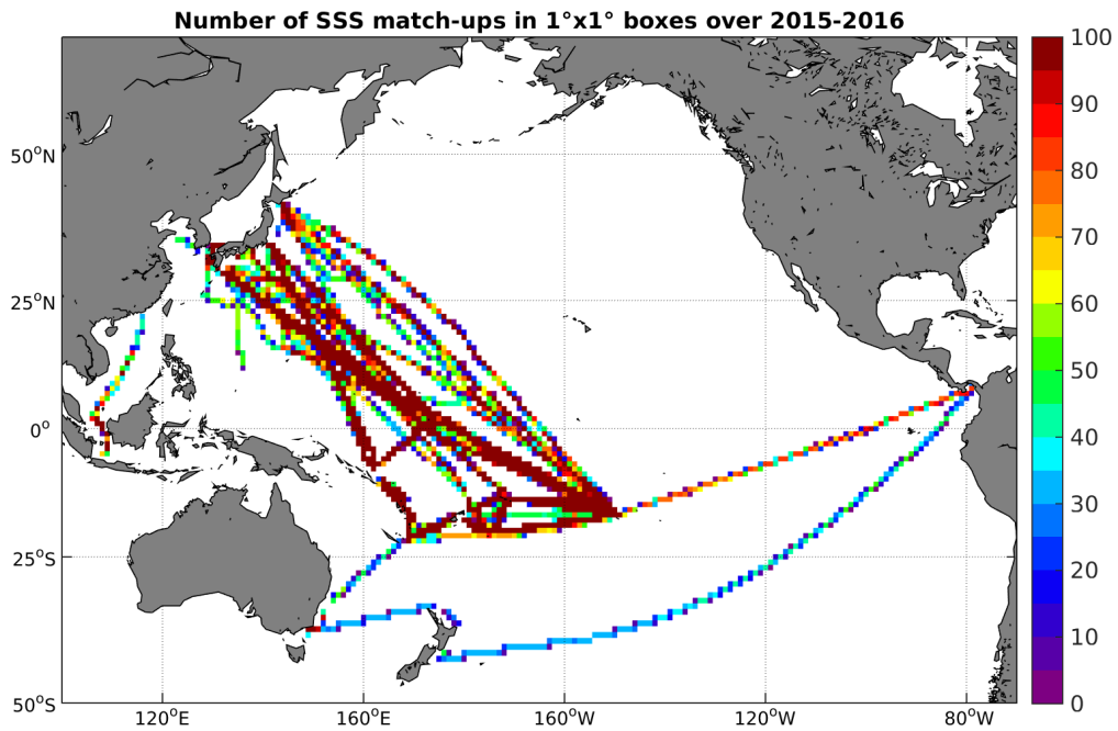
Figure 4: Number of SSS match-ups between TSG-LEGOS-DM SSS and the SMAP-L3-RSS-V2-MONTHLY-0.25DEG-40KM SSS product for the Pacific Ocean Pi-MEP region over 1^\circ \times 1^\circ boxes and for the full satellite product period.
