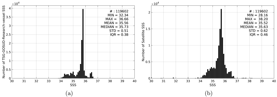
Figure 2: Histograms of SSS from TSG-GOSUD-Research-vessel (a) and SMAP-L3-RSS-V2-MONTHLY-0.25DEG-40KM (b) considering all match-up pairs per bins of 0.1 over the Pacific Ocean Pi-MEP region and for the full satellite product period.
