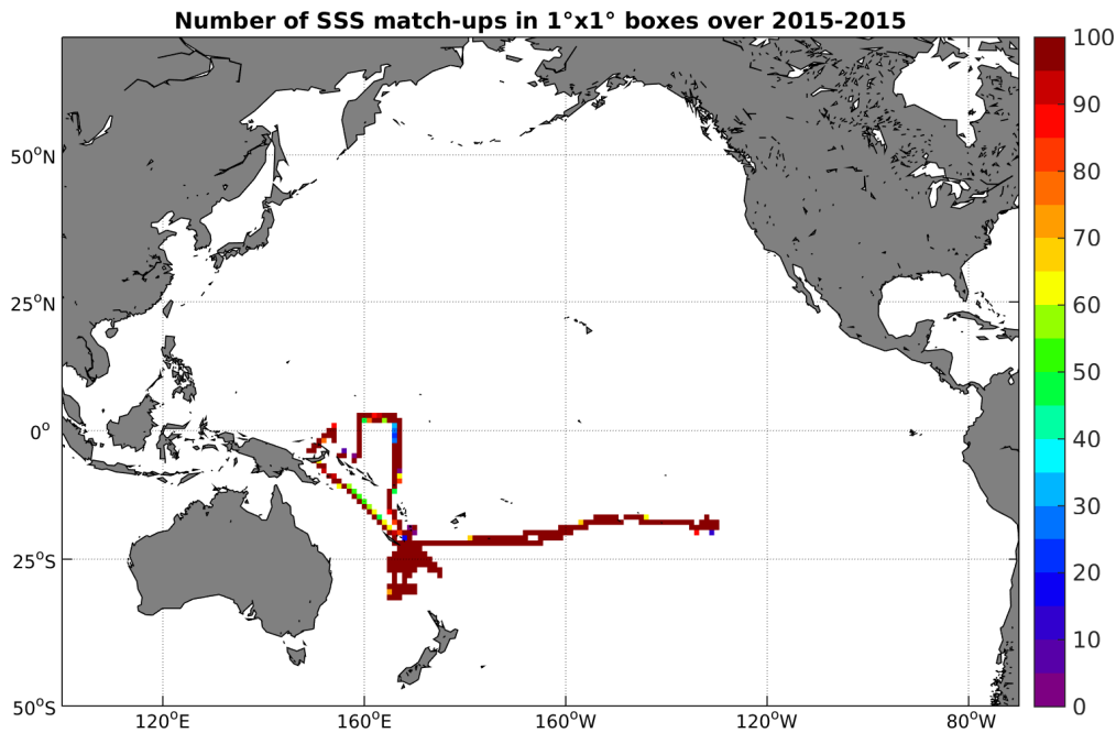
Figure 4: Number of SSS match-ups between TSG-GOSUD-Research-vessel SSS and the SMAP-L3-RSS-V2-MONTHLY-0.25DEG-40KM SSS product for the Pacific Ocean Pi-MEP region over 1^\circ \times 1^\circ boxes and for the full satellite product period.
