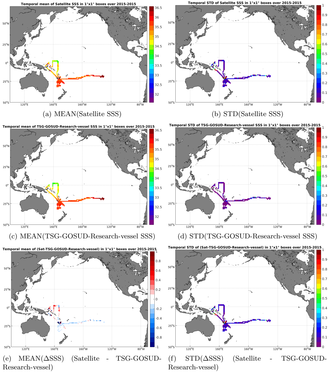
Figure 6: Temporal mean (left) and STD (right) of SSS from SMAP-L3-RSS-V2-MONTHLY-0.25DEG-40KM (top), TSG-GOSUD-Research-vessel (middle), and of \Delta SSS (Satellite - TSG-GOSUD-Research-vessel). Only match-up pairs are used to generate these maps.
