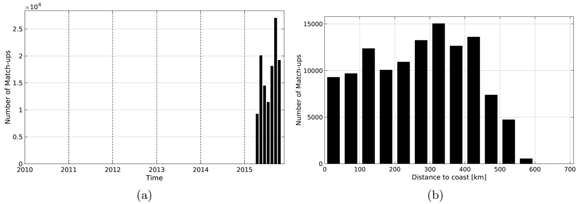
Figure 1: Number of match-ups between TSG-GOSUD-Research-vessel and SMAP-L3-RSS-V2-MONTHLY-0.25DEG-40KM SSS as a function of time (a) and as function of the distance to coast (b) over the Pacific Ocean Pi-MEP region and for the full satellite product period.
