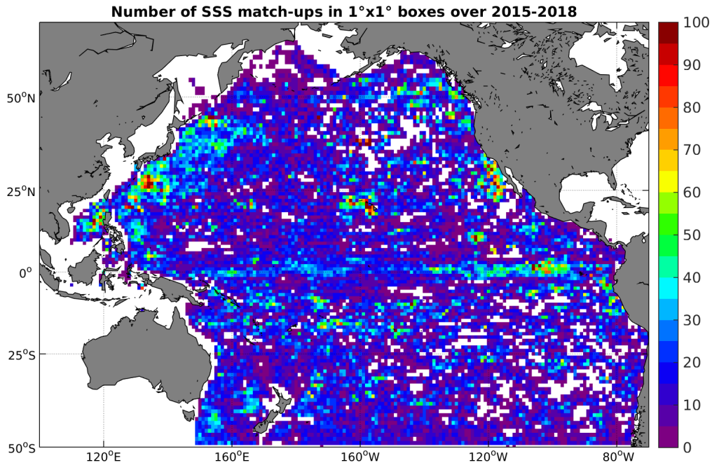
Figure 4: Number of SSS match-ups between Argo SSS and the SMAP-L3-RSS-V2-MONTHLY-0.25DEG-40KM SSS product for the Pacific Ocean Pi-MEP region over 1^\circ \times 1^\circ boxes and for the full satellite product period.
