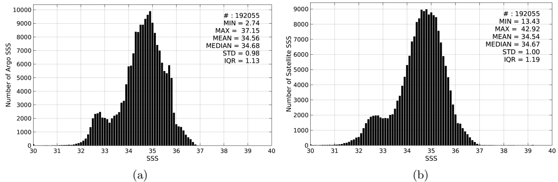
Figure 2: Histograms of SSS from Argo (a) and SMAP-L3-RSS-V2-MONTHLY-0.25DEG-40KM (b) considering all match-up pairs per bins of 0.1 over the Pacific Ocean Pi-MEP region and for the full satellite product period.
