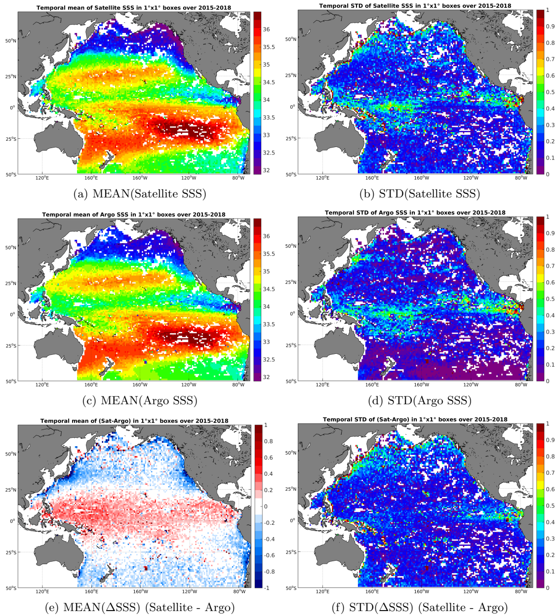
Figure 6: Temporal mean (left) and STD (right) of SSS from SMAP-L3-RSS-V2-MONTHLY-0.25DEG-40KM (top), Argo (middle), and of \Delta SSS (Satellite - Argo). Only match-up pairs are used to generate these maps.
