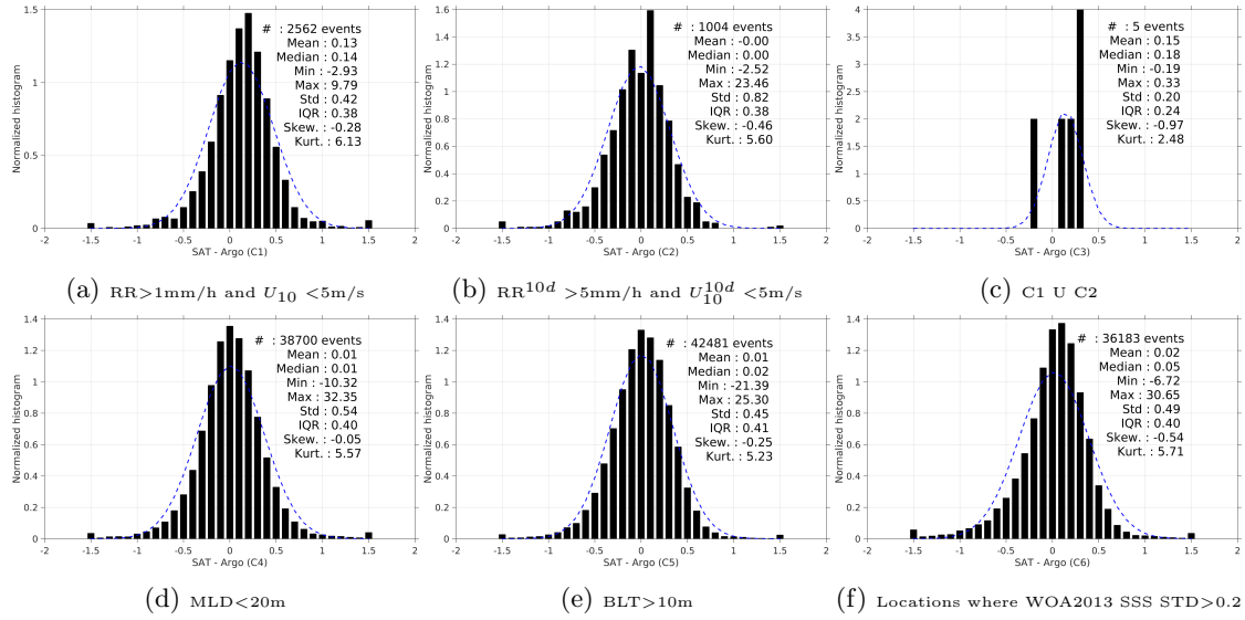
Figure 13: Normalized histogram of \Delta\text{SSS} (SMAP-L3-RSS-V2-MONTHLY-0.25DEG-40KM - Argo) for 6 different subdatasets corresponding to: RR>1mm/h and U_{10} < 5\text{m/s} (a), RR^{10d} > 5\text{mm/h} and U_{10}^{10d} < 5\text{m/s} (b), C1 U C2 (c),MLD<20m (d),BLT>10m (e),Locations where WOA2013 SSS STD>0.2 (f).
