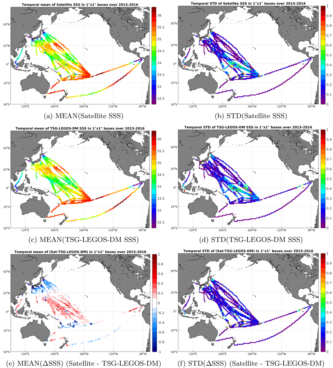
Figure 6: Temporal mean (left) and STD (right) of SSS from SMAP-L3-RSS-V2-MONTHLY-70KM (top), TSG-LEGOS-DM (middle), and of \Delta SSS (Satellite - TSG-LEGOS-DM). Only match-up pairs are used to generate these maps.
