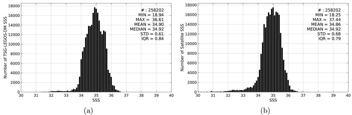
Figure 2: Histograms of SSS from TSG-LEGOS-DM (a) and SMAP-L3-RSS-V2-MONTHLY-70KM (b) considering all match-up pairs per bins of 0.1 over the Pacific Ocean Pi-MEP region and for the full satellite product period.
