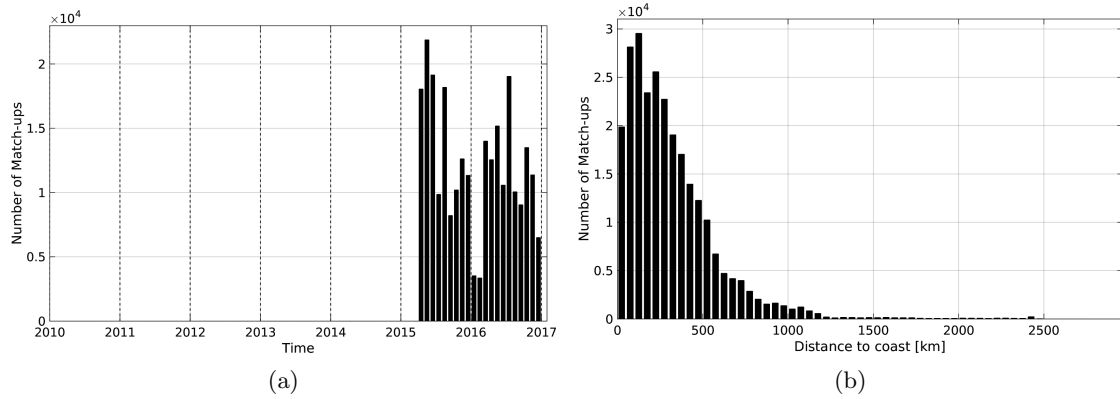
Figure 1: Number of match-ups between TSG-LEGOS-DM and SMAP-L3-RSS-V2-MONTHLY-70KM SSS as a function of time (a) and as function of the distance to coast (b) over the Pacific Ocean Pi-MEP region and for the full satellite product period.
