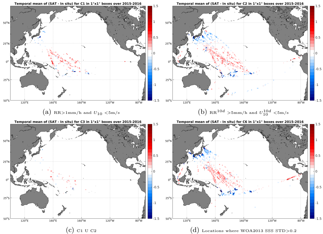
Figure 12: Temporal mean gridded over spatial boxes of size 1^\circ \times 1^\circ of \Delta SSS (SMAP-L3-RSS-V2-MONTHLY-70KM - TSG-LEGOS-DM) for 4 different subdatasets corresponding to: RR > 1\text{mm/h} and U_{10} < 5\text{m/s} (a), RR^{10d} > 5\text{mm/h} and U_{10}^{10d} < 5\text{m/s} (b), C1 U C2 (c), Locations where WOA2013 SSS STD > 0.2 (d).
