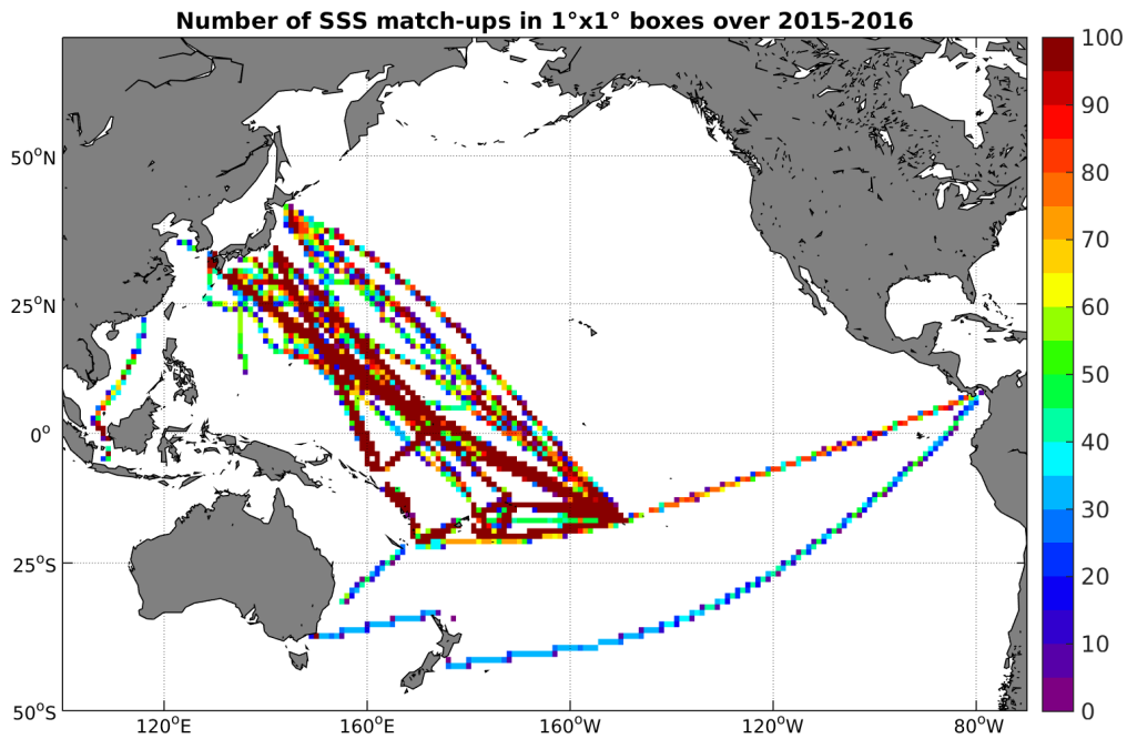
Figure 4: Number of SSS match-ups between TSG-LEGOS-DM SSS and the SMAP-L3-RSS-V2-MONTHLY-70KM SSS product for the Pacific Ocean Pi-MEP region over 1^\circ \times 1^\circ boxes and for the full satellite product period.
