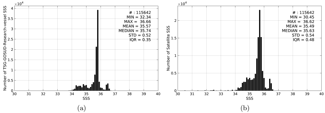
Figure 2: Histograms of SSS from TSG-GOSUD-Research-vessel (a) and SMAP-L3-RSS-V2-MONTHLY-70KM (b) considering all match-up pairs per bins of 0.1 over the Pacific Ocean Pi-MEP region and for the full satellite product period.
