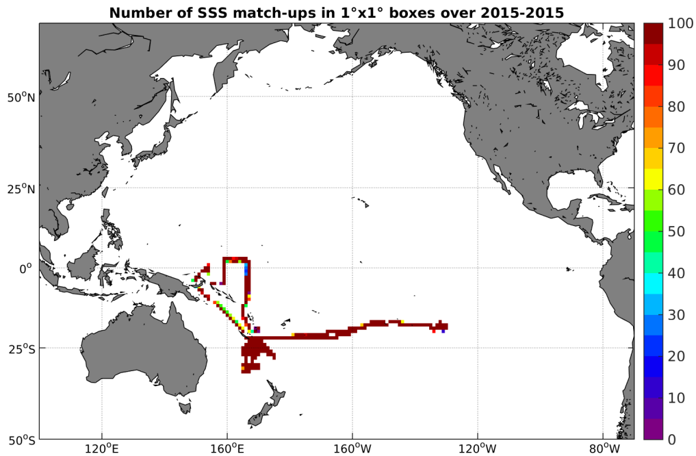
Figure 4: Number of SSS match-ups between TSG-GOSUD-Research-vessel SSS and the SMAP-L3-RSS-V2-MONTHLY-70KM SSS product for the Pacific Ocean Pi-MEP region over 1^\circ \times 1^\circ boxes and for the full satellite product period.
