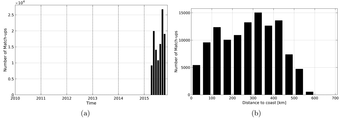
Figure 1: Number of match-ups between TSG-GOSUD-Research-vessel and SMAP-L3-RSS-V2-MONTHLY-70KM SSS as a function of time (a) and as function of the distance to coast (b) over the Pacific Ocean Pi-MEP region and for the full satellite product period.
