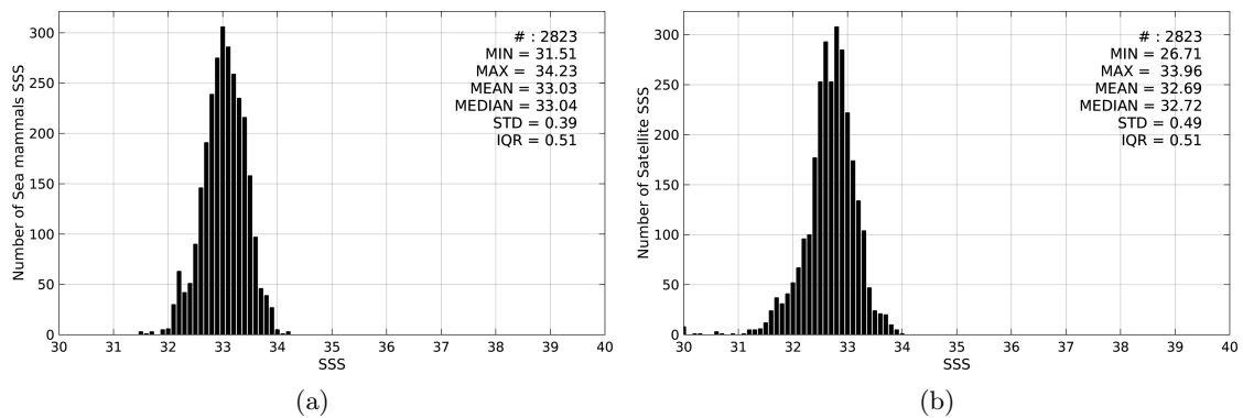
Figure 2: Histograms of SSS from Sea mammals (a) and SMAP-L3-RSS-V2-MONTHLY-70KM (b) considering all match-up pairs per bins of 0.1 over the Pacific Ocean Pi-MEP region and for the full satellite product period.
