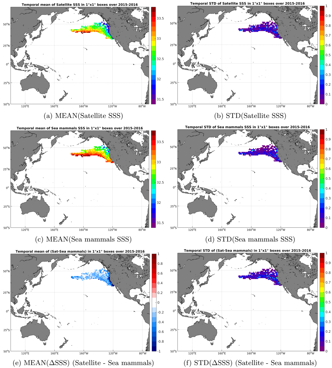
Figure 6: Temporal mean (left) and STD (right) of SSS from SMAP-L3-RSS-V2-MONTHLY-70KM (top), Sea mammals (middle), and of \Delta SSS (Satellite - Sea mammals). Only match-up pairs are used to generate these maps.
