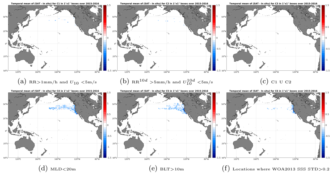
Figure 12: Temporal mean gridded over spatial boxes of size 1^\circ \times 1^\circ of \Delta SSS (SMAP-L3-RSS-V2-MONTHLY-70KM - Sea mammals) for 6 different subdatasets corresponding to:RR>1mm/h and U_{10} < 5\text{m/s} (a), RR^{10d} > 5\text{mm/h} and U_{10}^{10d} < 5\text{m/s} (b), C1 U C2 (c),MLD<20m (d),BLT>10m (e),Locations where WOA2013 SSS STD>0.2 (f).
