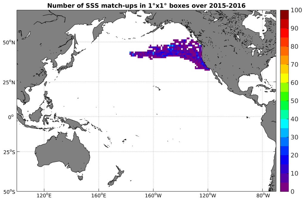
Figure 4: Number of SSS match-ups between Sea mammals SSS and the SMAP-L3-RSS-V2-MONTHLY-70KM SSS product for the Pacific Ocean Pi-MEP region over 1^\circ \times 1^\circ boxes and for the full satellite product period.
