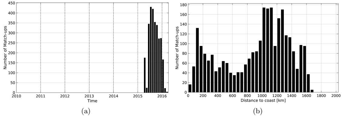
Figure 1: Number of match-ups between Sea mammals and SMAP-L3-RSS-V2-MONTHLY-70KM SSS as a function of time (a) and as function of the distance to coast (b) over the Pacific Ocean Pi-MEP region and for the full satellite product period.
