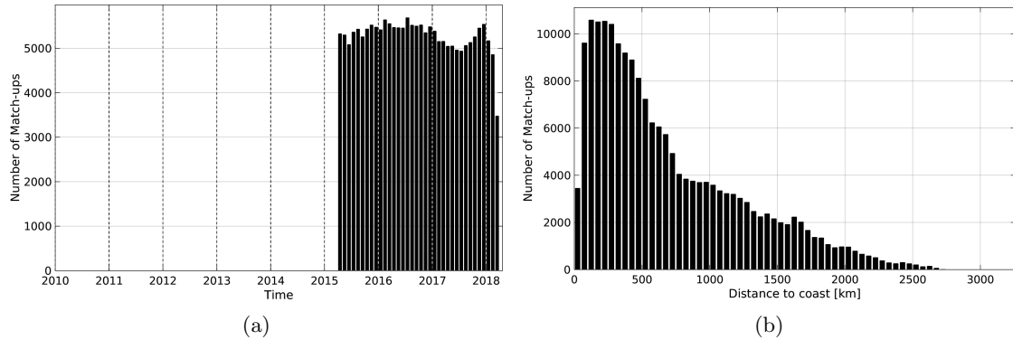
Figure 1: Number of match-ups between Argo and SMAP-L3-RSS-V2-MONTHLY-70KM SSS as a function of time (a) and as function of the distance to coast (b) over the Pacific Ocean Pi-MEP region and for the full satellite product period.
