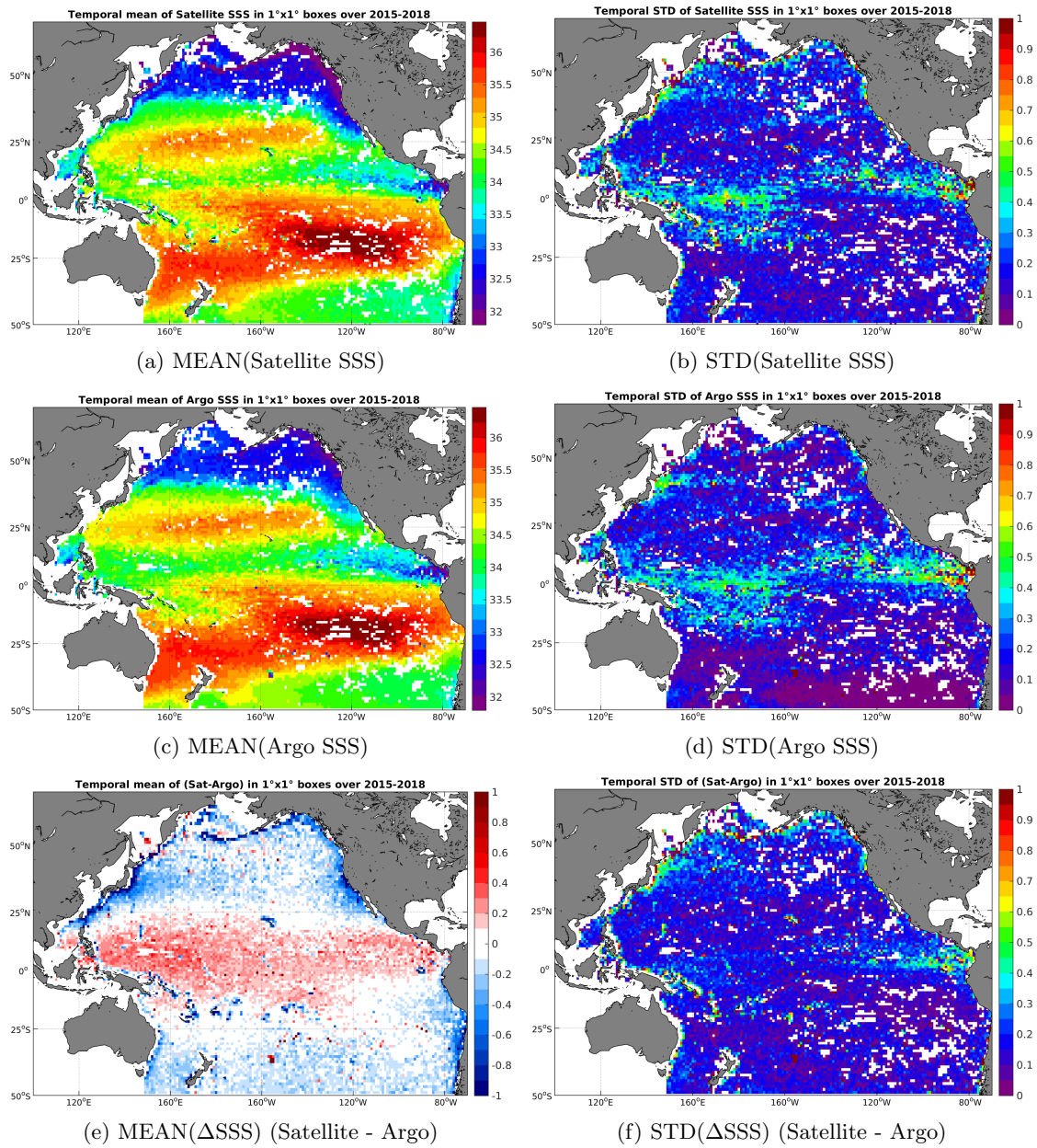
Figure 6: Temporal mean (left) and STD (right) of SSS from SMAP-L3-RSS-V2-MONTHLY-70KM (top), Argo (middle), and of \Delta SSS (Satellite - Argo). Only match-up pairs are used to generate these maps.
