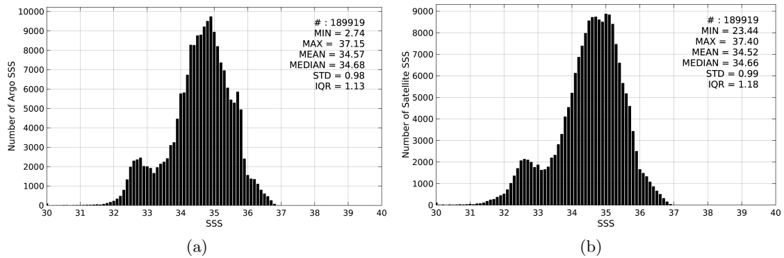
Figure 2: Histograms of SSS from Argo (a) and SMAP-L3-RSS-V2-MONTHLY-70KM (b) considering all match-up pairs per bins of 0.1 over the Pacific Ocean Pi-MEP region and for the full satellite product period.
