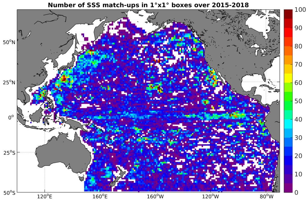
Figure 4: Number of SSS match-ups between Argo SSS and the SMAP-L3-RSS-V2-MONTHLY-70KM SSS product for the Pacific Ocean Pi-MEP region over 1°x1° boxes and for the full satellite product period.
