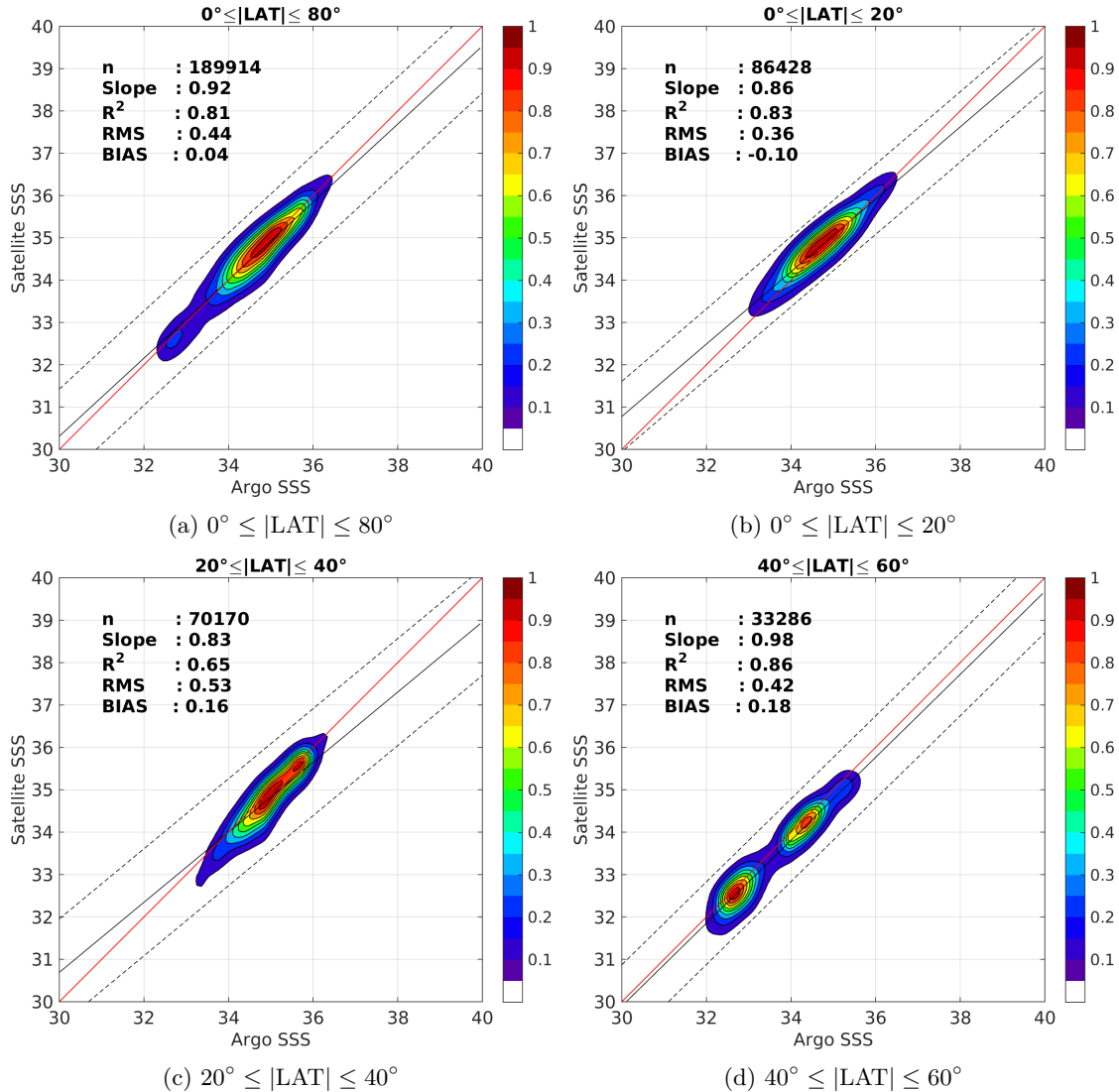
Figure 9: Contour maps of the concentration of SMAP-L3-RSS-V2-MONTHLY-70KM SSS (y-axis) versus Argo SSS (x-axis) at match-up pairs for different latitude bands. For each plot, the red line shows x=y . The black thin and dashed lines indicate a linear fit through the data cloud and the \pm 95\% confidence levels, respectively. The number match-up pairs n , the slope and R^2 coefficient of the linear fit, the root mean square (RMS) and the mean bias between satellite and in situ data are indicated for each latitude band in each plots.
