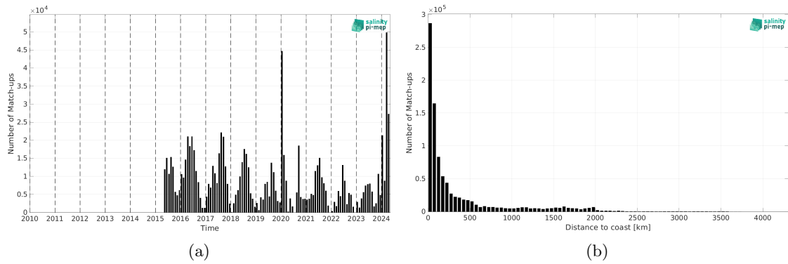
Figure 2: Number of match-ups between TSG (SAMOS) and SMAP SSS L3 v5.0 - 8-Day running (JPL) SSS as a function of time (a) and as function of the distance to coast (b) over the Pacific Ocean Pi-MEP region and for the full satellite product period.
