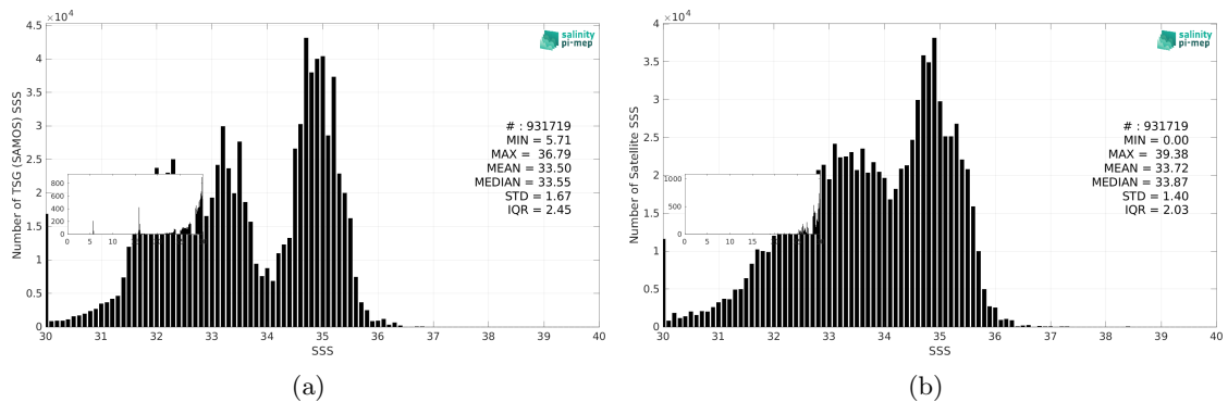
Figure 3: Histograms of SSS from TSG (SAMOS) (a) and SMAP SSS L3 v5.0 - 8-Day running (JPL) (b) considering all match-up pairs per bins of 0.1 over the Pacific Ocean Pi-MEP region and for the full satellite product period.
