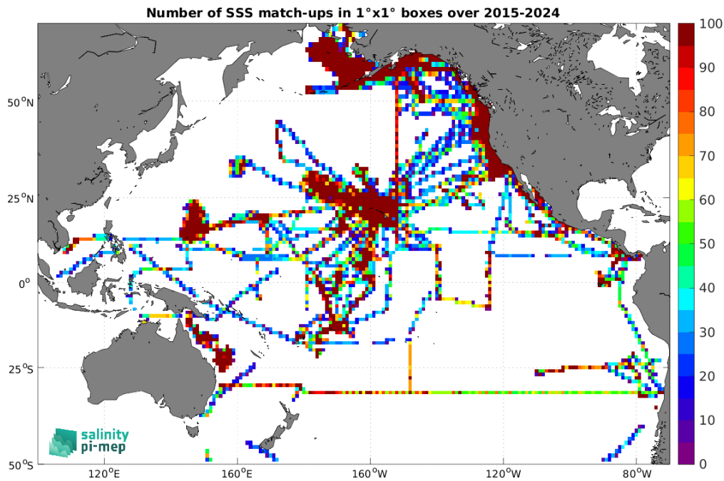
Figure 5: Number of SSS match-ups between TSG (SAMOS) SSS and the SMAP SSS L3 v5.0 - 8-Day running (JPL) SSS product for the Pacific Ocean Pi-MEP region over 1^\circ \times 1^\circ boxes and for the full satellite product period.
