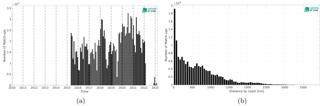
Figure 2: Number of match-ups between TSG (LEGOS-DM) and SMAP SSS L3 v5.0 - 8-Day running (JPL) SSS as a function of time (a) and as function of the distance to coast (b) over the Pacific Ocean Pi-MEP region and for the full satellite product period.
