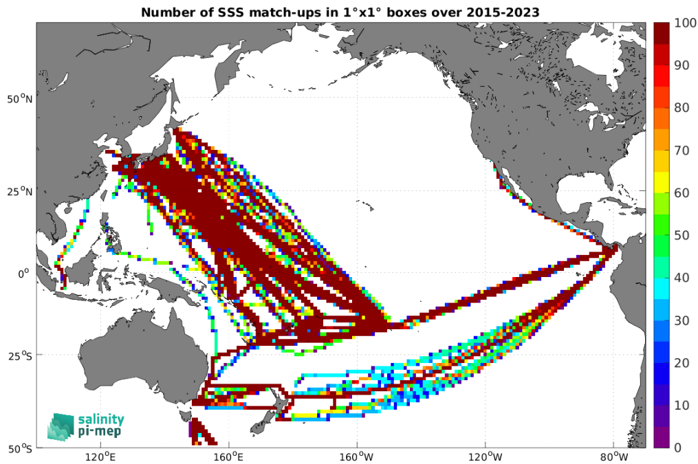
Figure 5: Number of SSS match-ups between TSG (LEGOS-DM) SSS and the SMAP SSS L3 v5.0 - 8-Day running (JPL) SSS product for the Pacific Ocean Pi-MEP region over 1^\circ \times 1^\circ boxes and for the full satellite product period.
