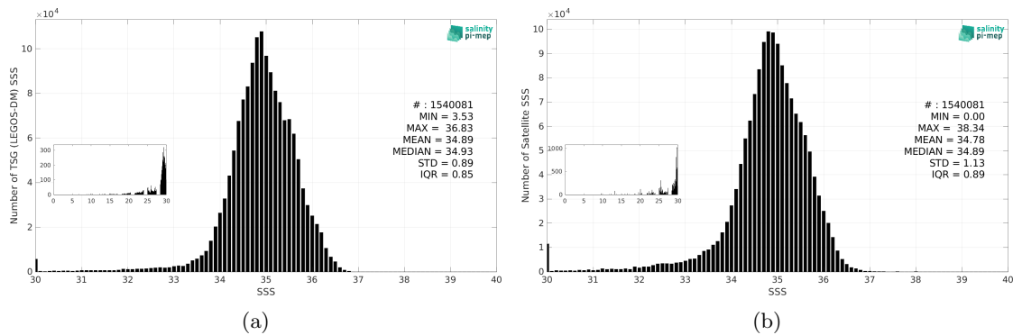
Figure 3: Histograms of SSS from TSG (LEGOS-DM) (a) and SMAP SSS L3 v5.0 - 8-Day running (JPL) (b) considering all match-up pairs per bins of 0.1 over the Pacific Ocean Pi-MEP region and for the full satellite product period.
