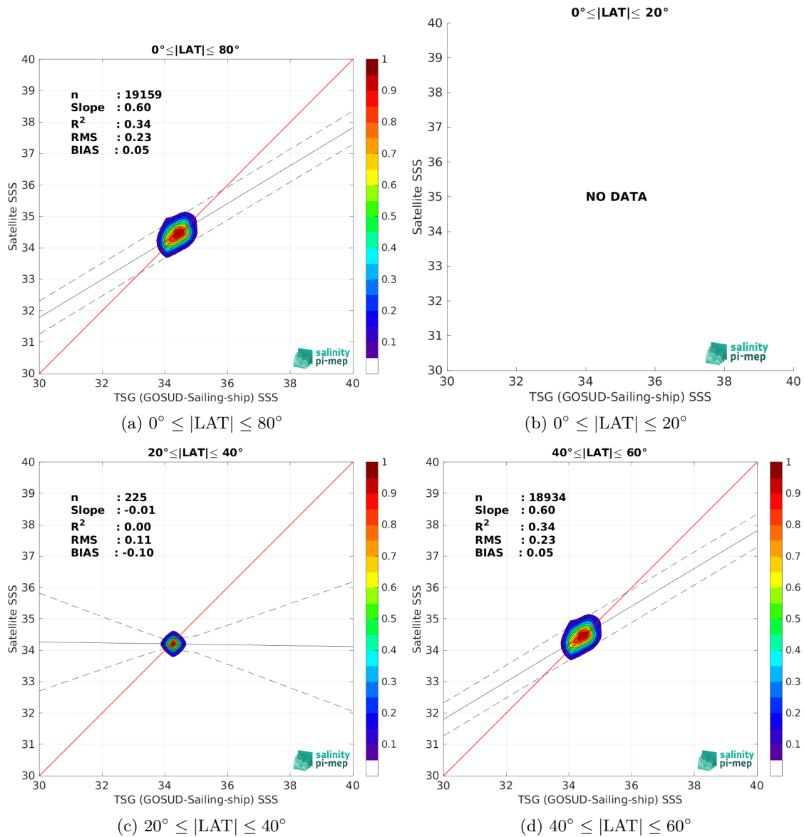
Figure 10: Contour maps of the concentration of SMAP SSS L3 v5.0 - 8-Day running (JPL) SSS (y-axis) versus TSG (GOSUD-Sailing-ship) SSS (x-axis) at match-up pairs for different latitude bands. For each plot, the red line shows x=y . The black thin and dashed lines indicate a linear fit through the data cloud and the \pm 95\% confidence levels, respectively. The number match-up pairs n , the slope and R^2 coefficient of the linear fit, the root mean square (RMS) and the mean bias between satellite and in situ data are indicated for each latitude band in each plots.
