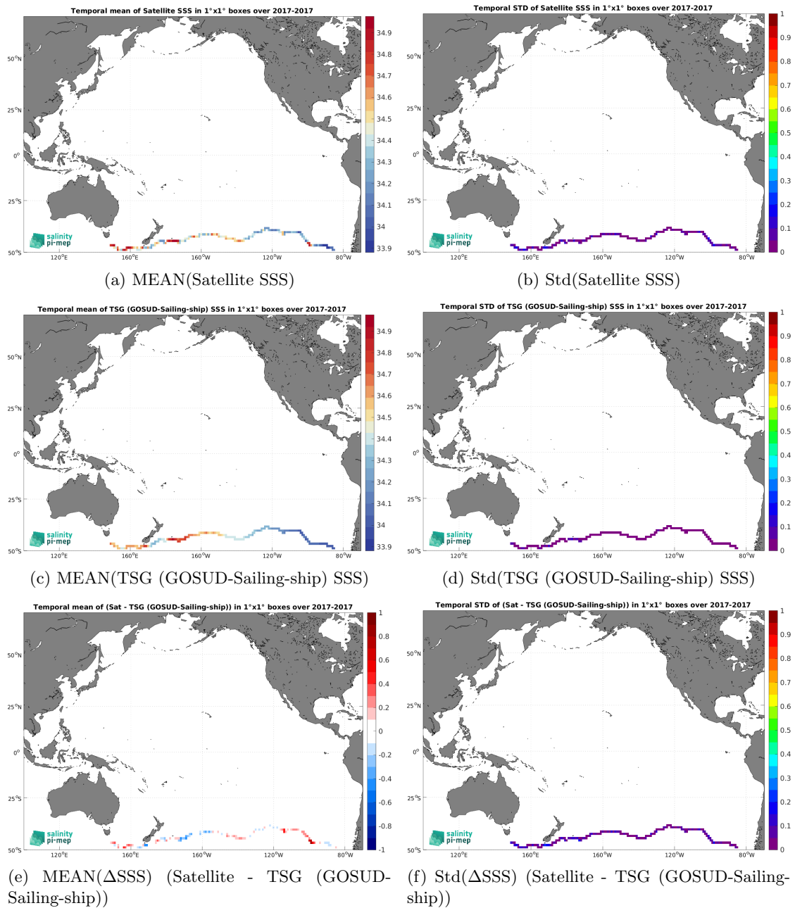
Figure 7: Temporal mean (left) and Std (right) of SSS from SMAP SSS L3 v5.0 - 8-Day running (JPL) (top), TSG (GOSUD-Sailing-ship) (middle), and of \Delta SSS (Satellite - TSG (GOSUD-Sailing-ship)). Only match-up pairs are used to generate these maps.
