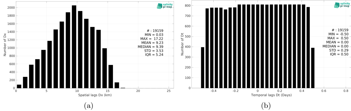
Figure 6: Histograms of the spatial (a) and temporal (b) lags between the location/time of the TSG (GOSUD-Sailing-ship) measurement and the date of the corresponding SMAP SSS L3 v5.0 - 8-Day running (JPL) SSS pixel.
