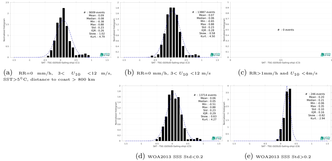
Figure 15: Normalized histogram of \Delta SSS (SMAP SSS L3 v5.0 - 8-Day running (JPL) - TSG (GOSUD-Sailing-ship)) for 5 different subdatasets corresponding to: RR=0 mm/h, 3 < U_{10} < 12 m/s, SST > 5°C, distance to coast > 800 km (a), RR=0 mm/h, 3 < U_{10} < 12 m/s (b), RR > 1mm/h and U_{10} < 4 m/s (c), WOA2013 SSS Std < 0.2 (d), WOA2013 SSS Std > 0.2 (e).
