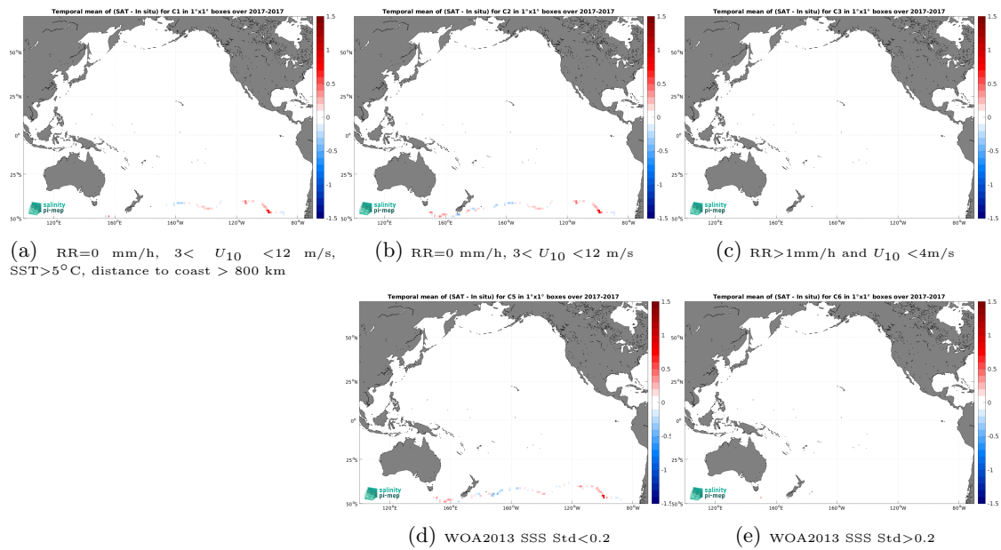
Figure 14: Temporal mean gridded over spatial boxes of size 1^\circ \times 1^\circ of \Delta SSS (SMAP SSS L3 v5.0 - 8-Day running (JPL) - TSG (GOSUD-Sailing-ship)) for 5 different subdatasets corresponding to:RR=0 mm/h, 3 < U_{10} < 12 m/s, SST >5^\circ C, distance to coast > 800 km (a), RR=0 mm/h, 3 < U_{10} < 12 m/s (b), RR >1 mm/h and U_{10} < 4 m/s (c), WOA2013 SSS Std <0.2 (d), WOA2013 SSS Std >0.2 (e).
