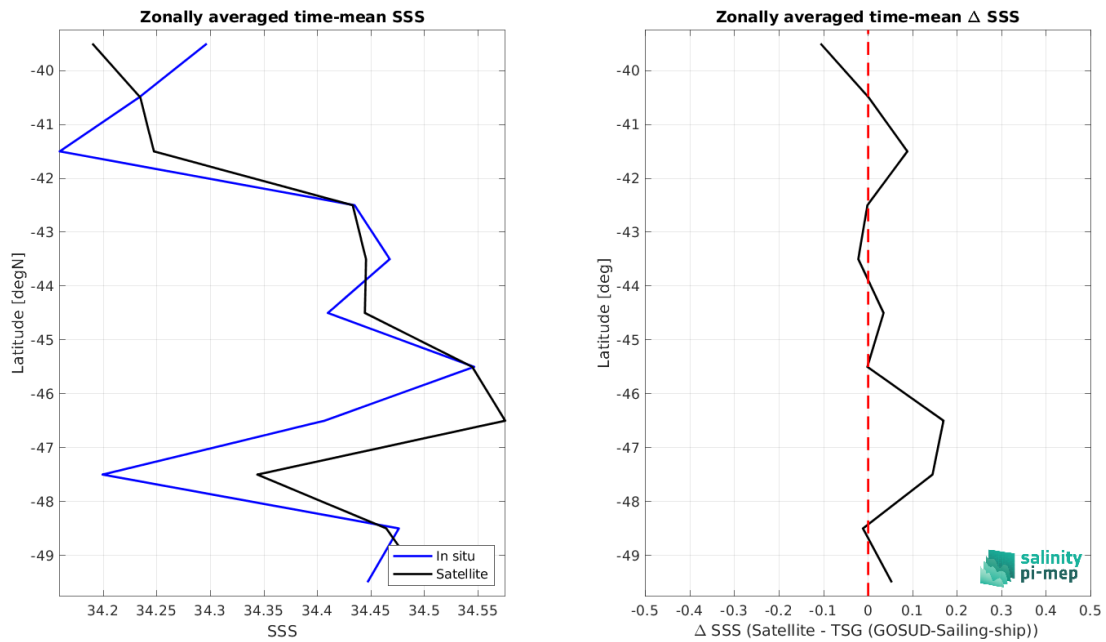
Figure 9: Left panel: Zonal mean SSS from SMAP SSS L3 v5.0 - 8-Day running (JPL) satellite product (black) and from TSG (GOSUD-Sailing-ship) (blue). Right panel: Zonal mean of \Delta SSS (Satellite - TSG (GOSUD-Sailing-ship)) for all the collected Pi-MEP match-up pairs estimated over the full satellite product period.
