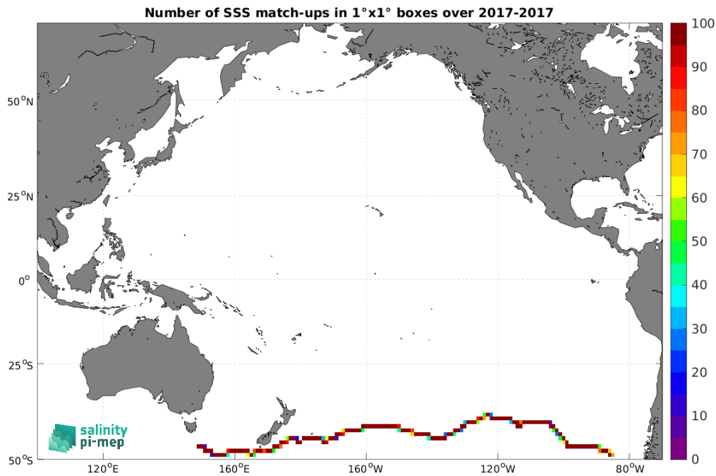
Figure 5: Number of SSS match-ups between TSG (GOSUD-Sailing-ship) SSS and the SMAP SSS L3 v5.0 - 8-Day running (JPL) SSS product for the Pacific Ocean Pi-MEP region over 1^\circ \times 1^\circ boxes and for the full satellite product period.
