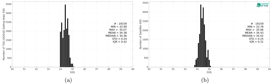
Figure 2: Histograms of SSS from TSG (GOSUD-Sailing-ship) (a) and SMAP SSS L3 v5.0 - 8-Day running (JPL) (b) considering all match-up pairs per bins of 0.1 over the Pacific Ocean Pi-MEP region and for the full satellite product period.
