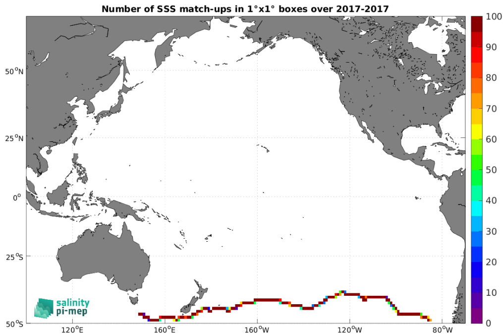
Figure 4: Number of SSS match-ups between TSG (GOSUD-Sailing-ship) SSS and the SMAP SSS L3 v5.0 - 8-Day running (JPL) SSS product for the Pacific Ocean Pi-MEP region over 1^\circ \times 1^\circ boxes and for the full satellite product period.
