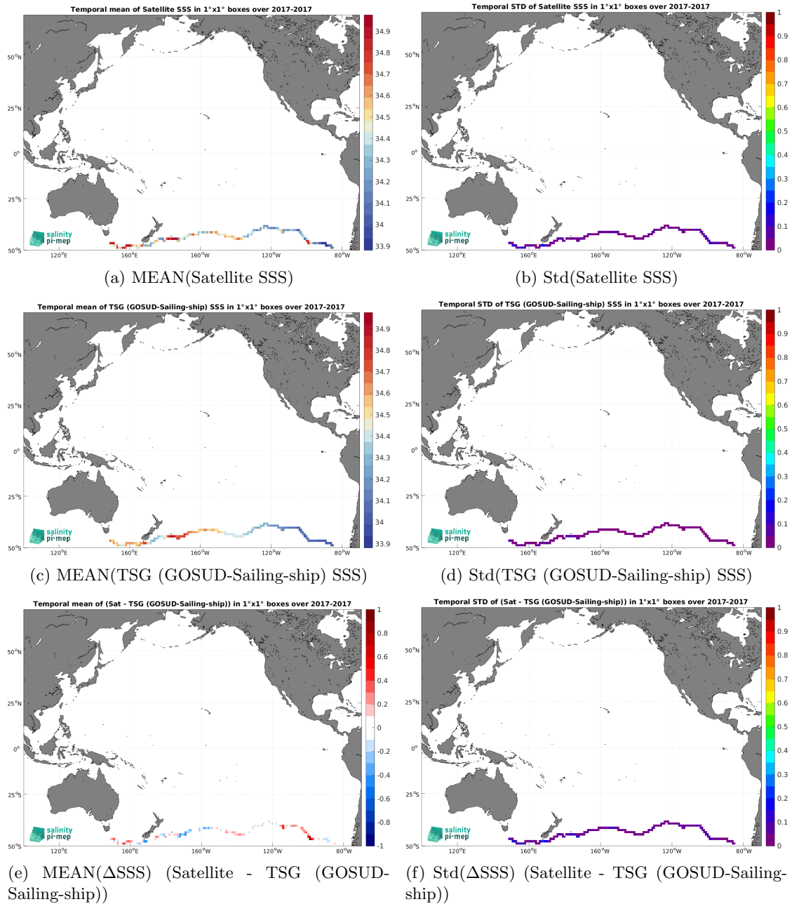
Figure 6: Temporal mean (left) and Std (right) of SSS from SMAP SSS L3 v5.0 - 8-Day running (JPL) (top), TSG (GOSUD-Sailing-ship) (middle), and of \Delta SSS (Satellite - TSG (GOSUD-Sailing-ship)). Only match-up pairs are used to generate these maps.
