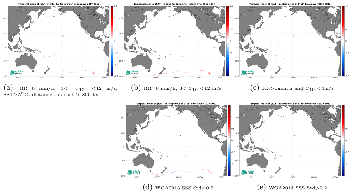
Figure 12: Temporal mean gridded over spatial boxes of size 1^\circ \times 1^\circ of \Delta SSS (SMAP SSS L3 v5.0 - 8-Day running (JPL) - TSG (GOSUD-Sailing-ship)) for 5 different subdatasets corresponding to:RR=0 mm/h, 3 < U_{10} < 12 m/s, SST >5^\circ C, distance to coast > 800 km (a), RR=0 mm/h, 3 < U_{10} < 12 m/s (b), RR >1 mm/h and U_{10} < 4 m/s (c), WOA2013 SSS Std <0.2 (d), WOA2013 SSS Std >0.2 (e).
