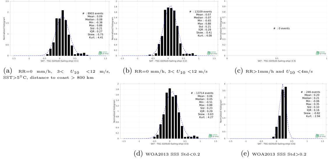
Figure 13: Normalized histogram of \Delta SSS (SMAP SSS L3 v5.0 - 8-Day running (JPL) - TSG (GOSUD-Sailing-ship)) for 5 different subdatasets corresponding to: RR=0 mm/h, 3 < U_{10} < 12 m/s, SST > 5°C, distance to coast > 800 km (a), RR=0 mm/h, 3 < U_{10} < 12 m/s (b), RR > 1mm/h and U_{10} < 4 m/s (c), WOA2013 SSS Std < 0.2 (d), WOA2013 SSS Std > 0.2 (e).
