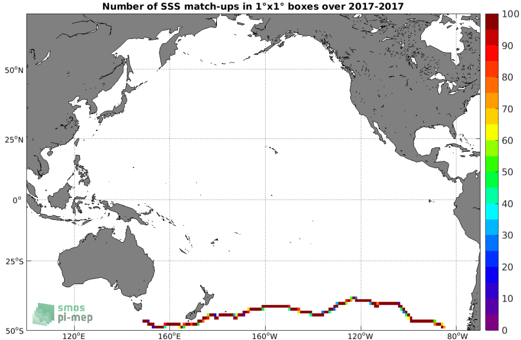
Figure 4: Number of SSS match-ups between TSG (GOSUD-Sailing-ship) SSS and the SMAP SSS L3 v5.0 - 8-Day running (JPL) SSS product for the Pacific Ocean Pi-MEP region over 1^\circ \times 1^\circ boxes and for the full satellite product period.
