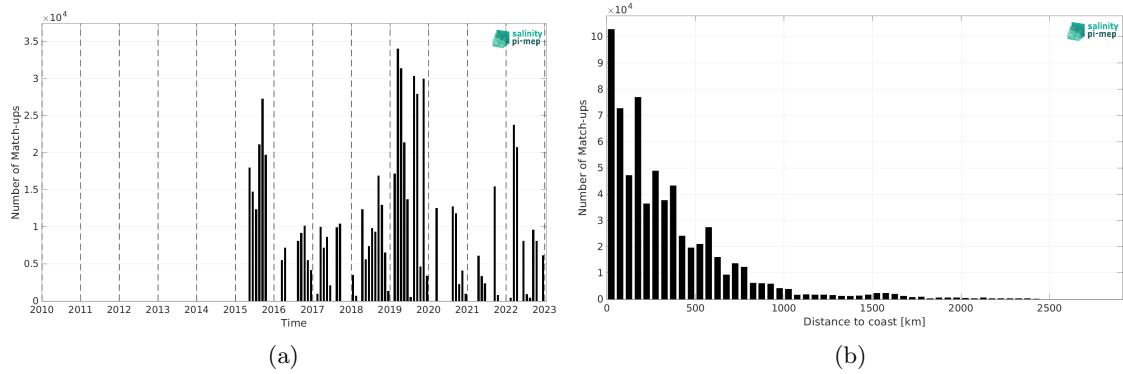
Figure 2: Number of match-ups between TSG (GOSUD-Research-vessel) and SMAP SSS L3 v5.0 - 8-Day running (JPL) SSS as a function of time (a) and as function of the distance to coast (b) over the Pacific Ocean Pi-MEP region and for the full satellite product period.
