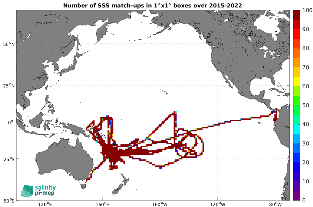
Figure 5: Number of SSS match-ups between TSG (GOSUD-Research-vessel) SSS and the SMAP SSS L3 v5.0 - 8-Day running (JPL) SSS product for the Pacific Ocean Pi-MEP region over 1^\circ \times 1^\circ boxes and for the full satellite product period.
