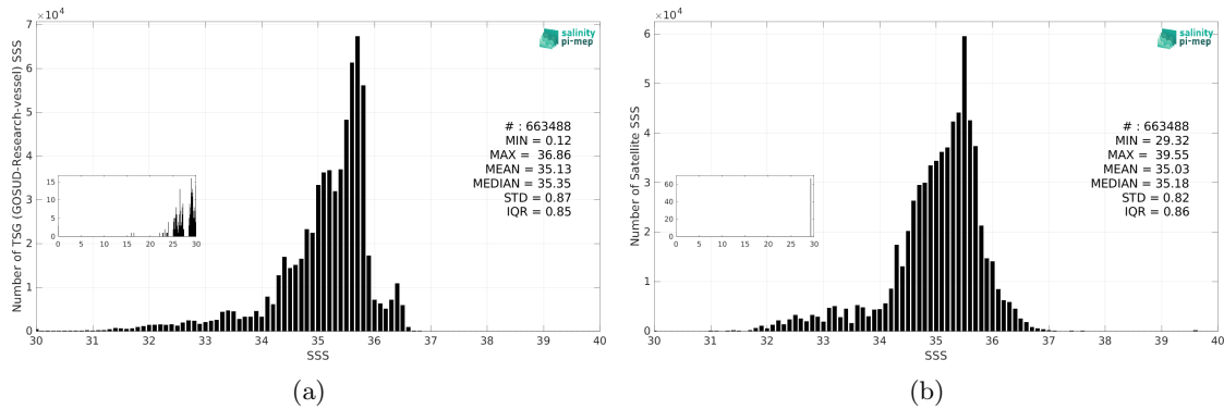
Figure 3: Histograms of SSS from TSG (GOSUD-Research-vessel) (a) and SMAP SSS L3 v5.0 - 8-Day running (JPL) (b) considering all match-up pairs per bins of 0.1 over the Pacific Ocean Pi-MEP region and for the full satellite product period.
